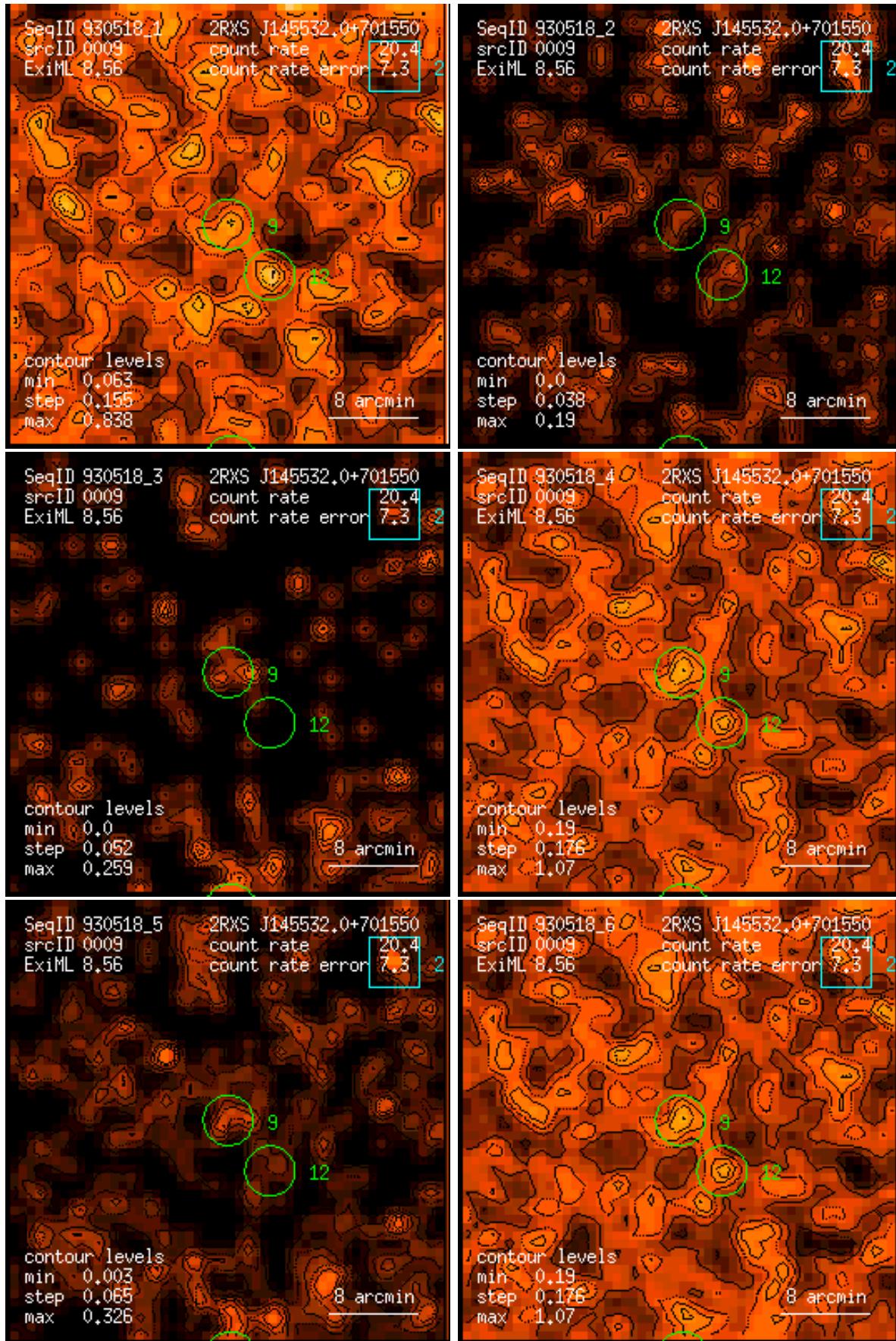
Figure 9: RASS 930518: detection 0009: band rate images, Gaussian filter: (1) PSPC channels 11 – 41, (2) 52 – 90, (3) 91 – 201, (4) 11 – 235, (5) 52 – 201, (6) 11 – 201. Broad band rates in counts/ks. Band rate contour levels in counts/ks/arcmin 2 .
