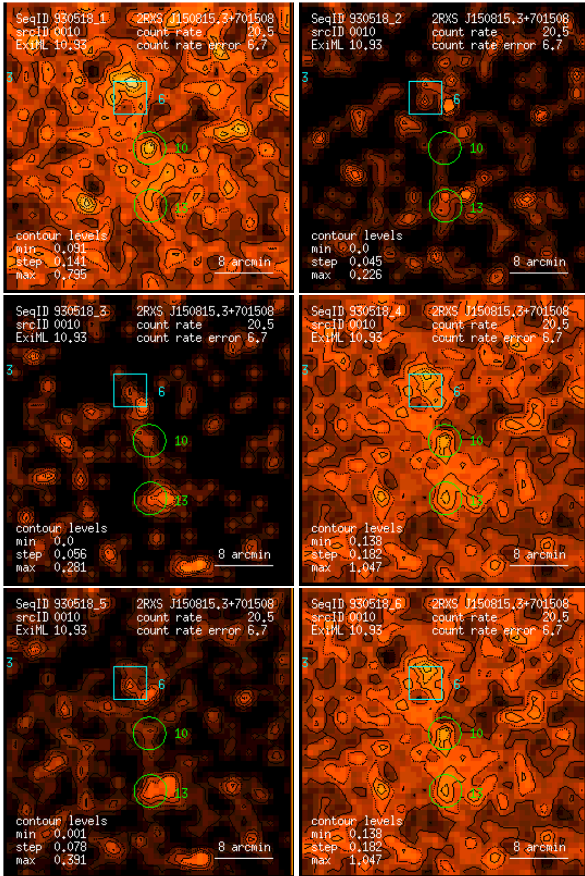
Figure 10: RASS 930518: detection 0010: band rate images, Gaussian filter: (1) PSPC channels 11 – 41, (2) 52 – 90, (3) 91 – 201, (4) 11 – 235, (5) 52 – 201, (6) 11 – 201. Broad band rates in counts/ks. Band rate contour levels in counts/ks/arcmin 2 .
