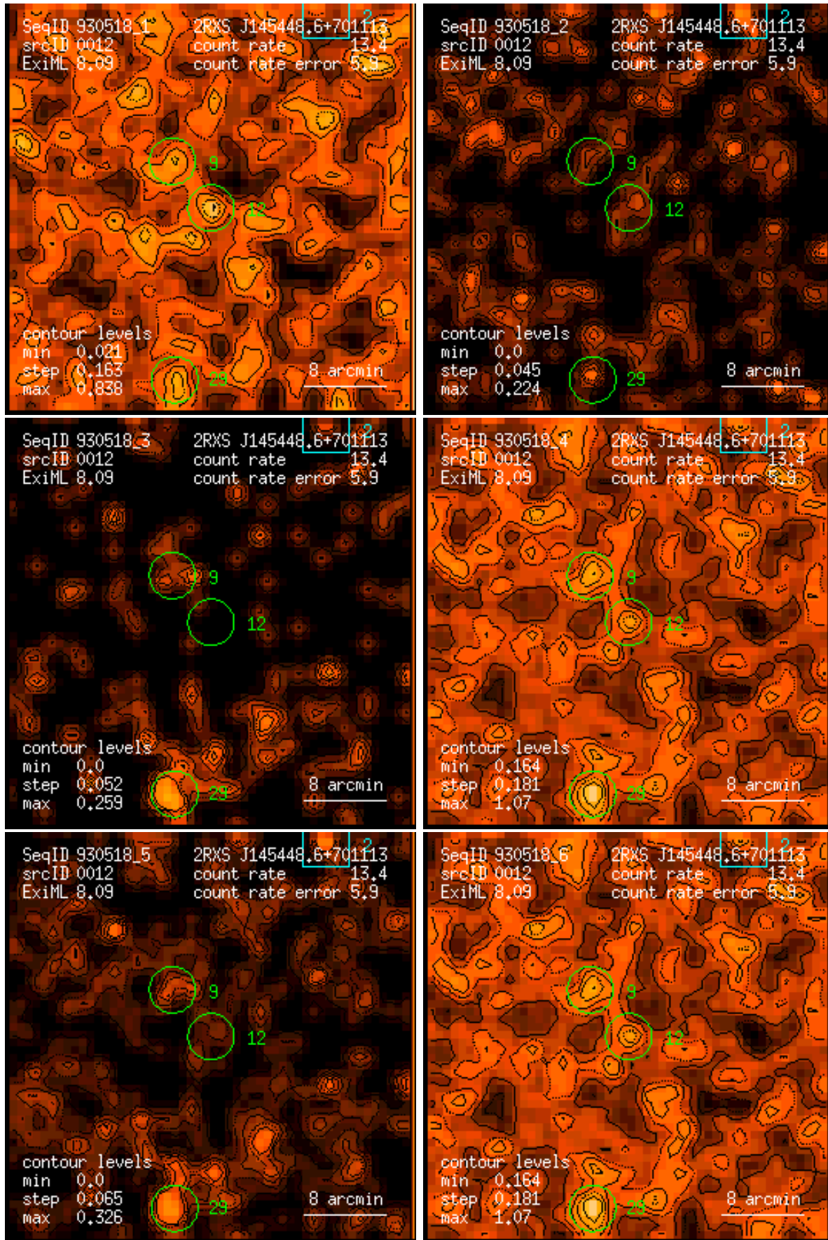
Figure 12: RASS 930518: detection 0012: band rate images, Gaussian filter: (1) PSPC channels 11 – 41, (2) 52 – 90, (3) 91 – 201, (4) 11 – 235, (5) 52 – 201, (6) 11 – 201. Broad band rates in counts/ks. Band rate contour levels in counts/ks/arcmin 2 .
