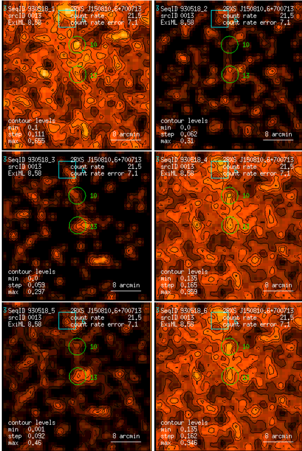
Figure 13: RASS 930518: detection 0013: band rate images, Gaussian filter: (1) PSPC channels 11 – 41, (2) 52 – 90, (3) 91 – 201, (4) 11 – 235, (5) 52 – 201, (6) 11 – 201. Broad band rates in counts/ks. Band rate contour levels in counts/ks/arcmin 2 .
