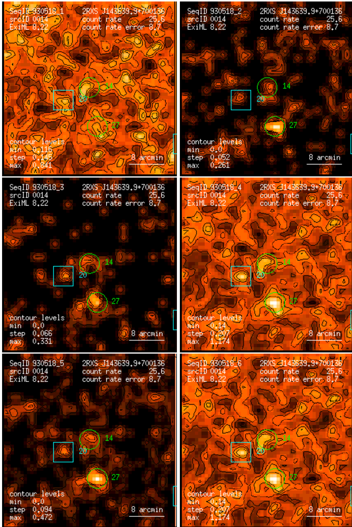
Figure 14: RASS 930518: detection 0014: band rate images, Gaussian filter: (1) PSPC channels 11 – 41, (2) 52 – 90, (3) 91 – 201, (4) 11 – 235, (5) 52 – 201, (6) 11 – 201. Broad band rates in counts/ks. Band rate contour levels in counts/ks/arcmin 2 .
