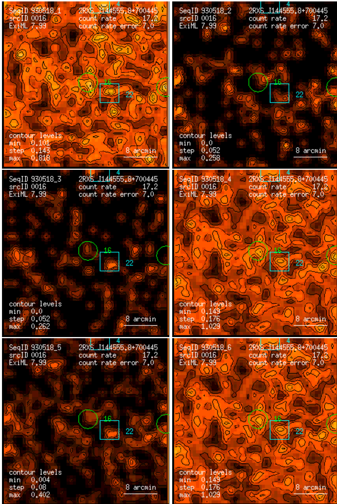
Figure 16: RASS 930518: detection 0016: band rate images, Gaussian filter: (1) PSPC channels 11 – 41, (2) 52 – 90, (3) 91 – 201, (4) 11 – 235, (5) 52 – 201, (6) 11 – 201. Broad band rates in counts/ks. Band rate contour levels in counts/ks/arcmin 2 .
