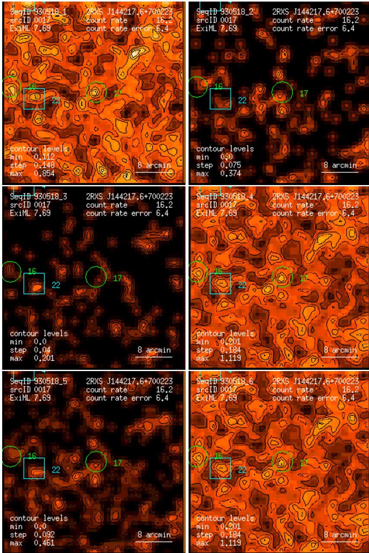
Figure 17: RASS 930518: detection 0017: band rate images, Gaussian filter: (1) PSPC channels 11 – 41, (2) 52 – 90, (3) 91 – 201, (4) 11 – 235, (5) 52 – 201, (6) 11 – 201. Broad band rates in counts/ks. Band rate contour levels in counts/ks/arcmin 2 .
