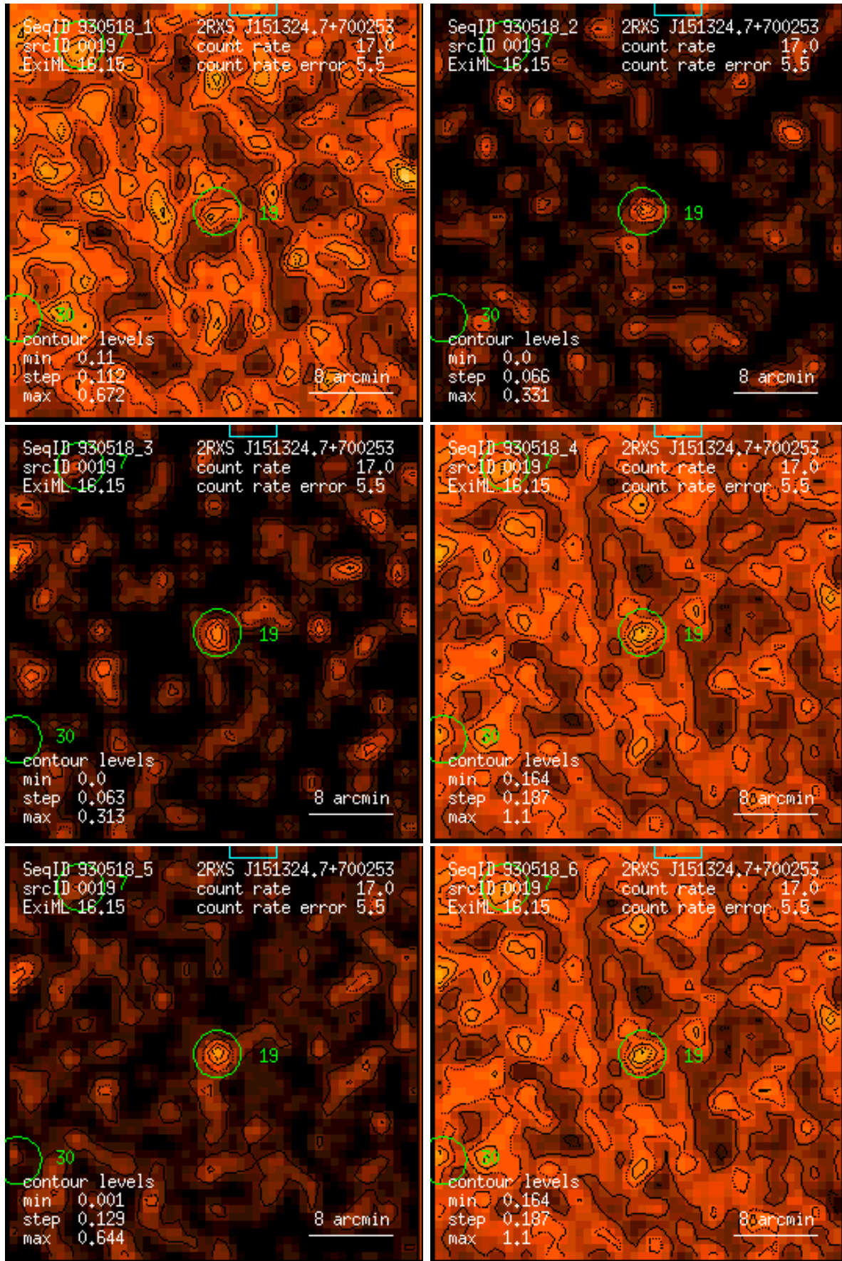
Figure 19: RASS 930518: detection 0019: band rate images, Gaussian filter: (1) PSPC channels 11 – 41, (2) 52 – 90, (3) 91 – 201, (4) 11 – 235, (5) 52 – 201, (6) 11 – 201. Broad band rates in counts/ks. Band rate contour levels in counts/ks/arcmin 2 .
