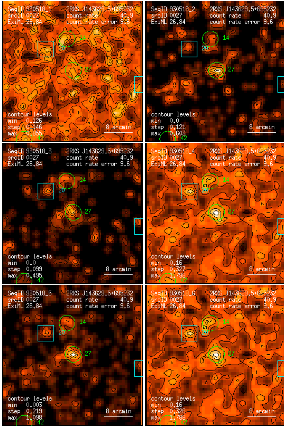
Figure 27: RASS 930518: detection 0027: band rate images, Gaussian filter: (1) PSPC channels 11 – 41, (2) 52 – 90, (3) 91 – 201, (4) 11 – 235, (5) 52 – 201, (6) 11 – 201. Broad band rates in counts/ks. Band rate contour levels in counts/ks/arcmin 2 .
