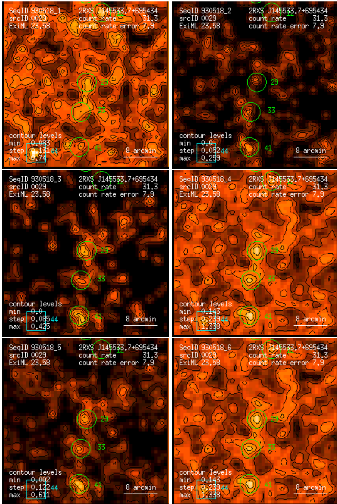
Figure 29: RASS 930518: detection 0029: band rate images, Gaussian filter: (1) PSPC channels 11 – 41, (2) 52 – 90, (3) 91 – 201, (4) 11 – 235, (5) 52 – 201, (6) 11 – 201. Broad band rates in counts/ks. Band rate contour levels in counts/ks/arcmin 2 .
