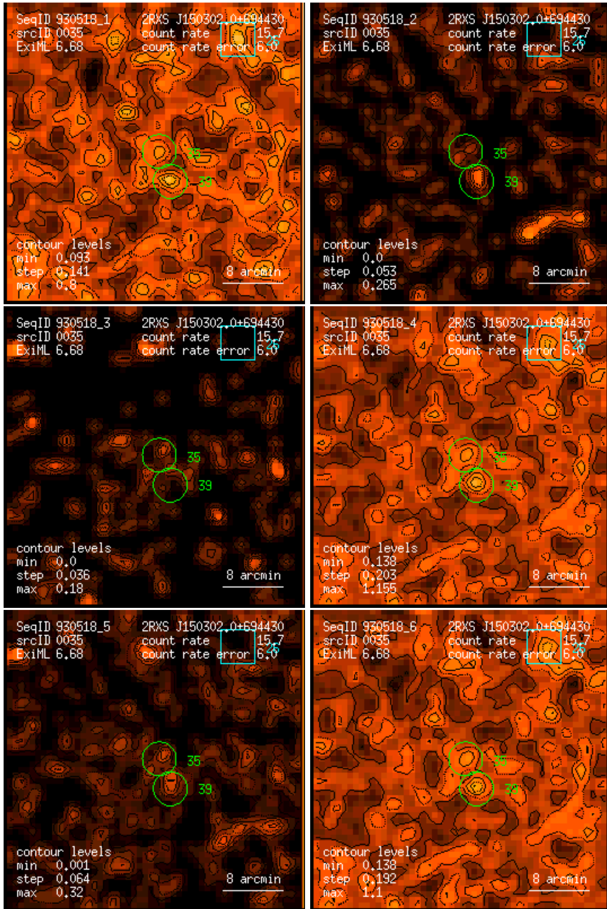
Figure 35: RASS 930518: detection 0035: band rate images, Gaussian filter: (1) PSPC channels 11 – 41, (2) 52 – 90, (3) 91 – 201, (4) 11 – 235, (5) 52 – 201, (6) 11 – 201. Broad band rates in counts/ks. Band rate contour levels in counts/ks/arcmin 2 .
