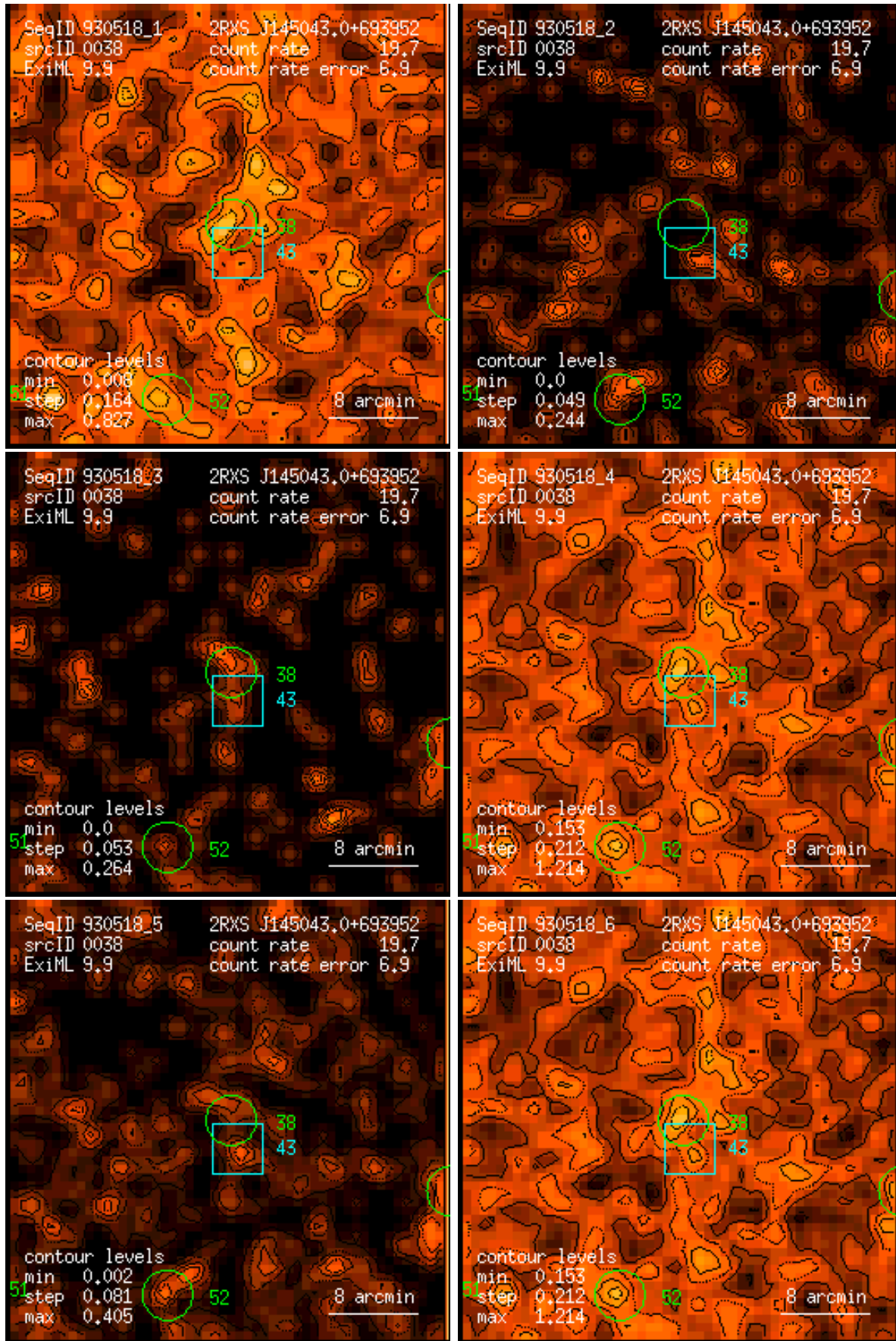
Figure 38: RASS 930518: detection 0038: band rate images, Gaussian filter: (1) PSPC channels 11 – 41, (2) 52 – 90, (3) 91 – 201, (4) 11 – 235, (5) 52 – 201, (6) 11 – 201. Broad band rates in counts/ks. Band rate contour levels in counts/ks/arcmin 2 .
