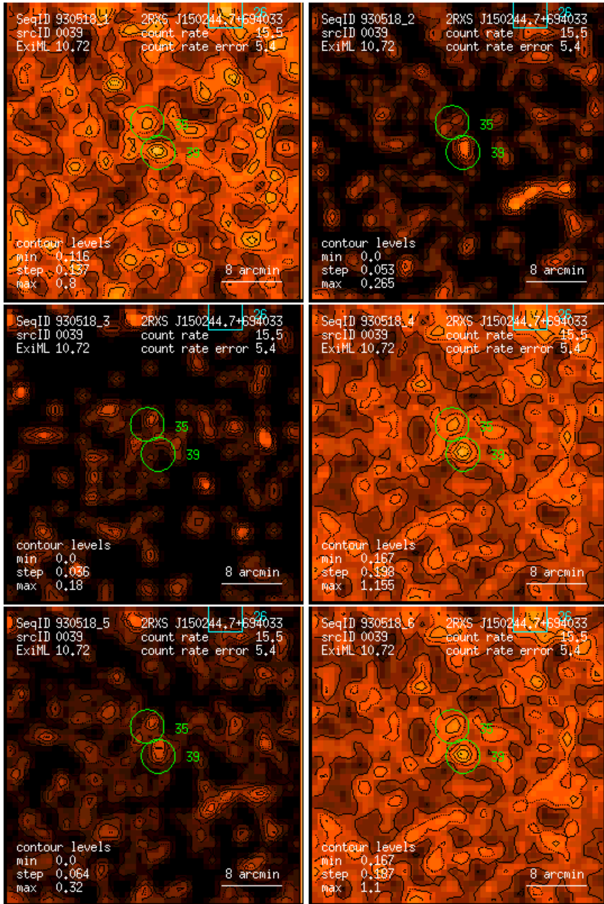
Figure 39: RASS 930518: detection 0039: band rate images, Gaussian filter: (1) PSPC channels 11 – 41, (2) 52 – 90, (3) 91 – 201, (4) 11 – 235, (5) 52 – 201, (6) 11 – 201. Broad band rates in counts/ks. Band rate contour levels in counts/ks/arcmin 2 .
