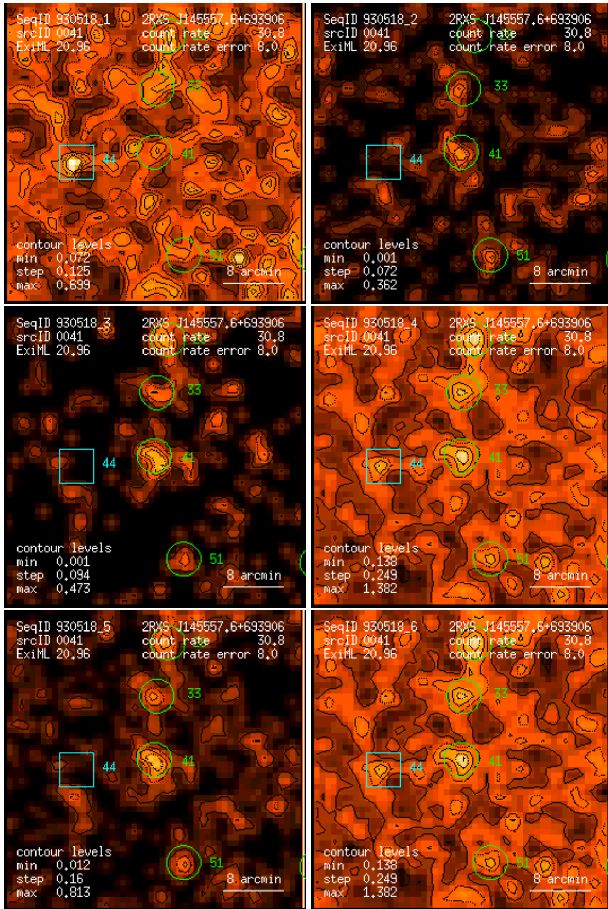
Figure 41: RASS 930518: detection 0041: band rate images, Gaussian filter: (1) PSPC channels 11 – 41, (2) 52 – 90, (3) 91 – 201, (4) 11 – 235, (5) 52 – 201, (6) 11 – 201. Broad band rates in counts/ks. Band rate contour levels in counts/ks/arcmin 2 .
