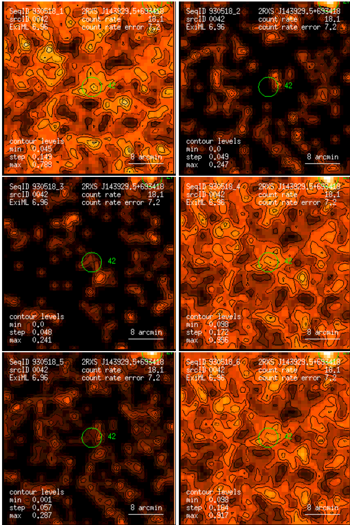
Figure 42: RASS 930518: detection 0042: band rate images, Gaussian filter: (1) PSPC channels 11 – 41, (2) 52 – 90, (3) 91 – 201, (4) 11 – 235, (5) 52 – 201, (6) 11 – 201. Broad band rates in counts/ks. Band rate contour levels in counts/ks/arcmin 2 .
