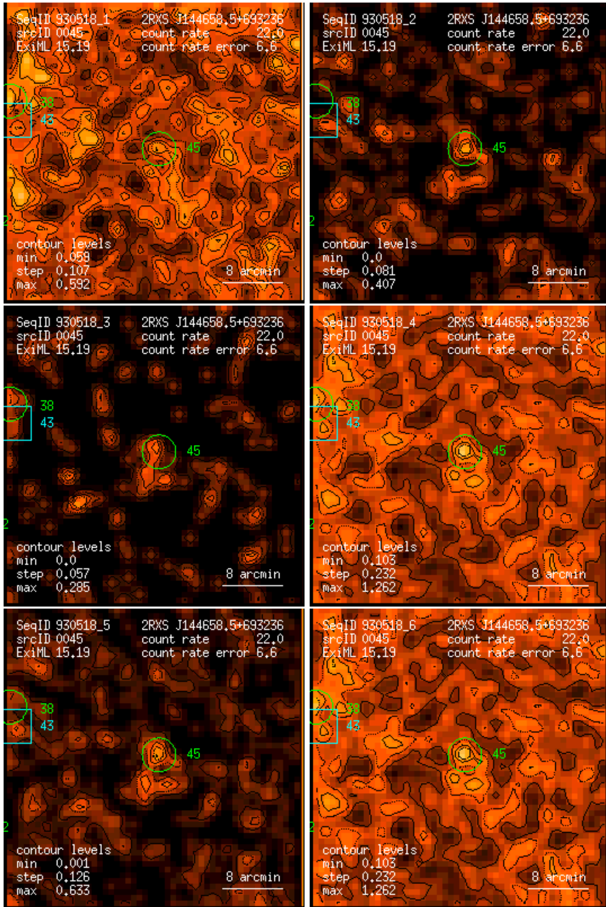
Figure 45: RASS 930518: detection 0045: band rate images, Gaussian filter: (1) PSPC channels 11 – 41, (2) 52 – 90, (3) 91 – 201, (4) 11 – 235, (5) 52 – 201, (6) 11 – 201. Broad band rates in counts/ks. Band rate contour levels in counts/ks/arcmin 2 .
