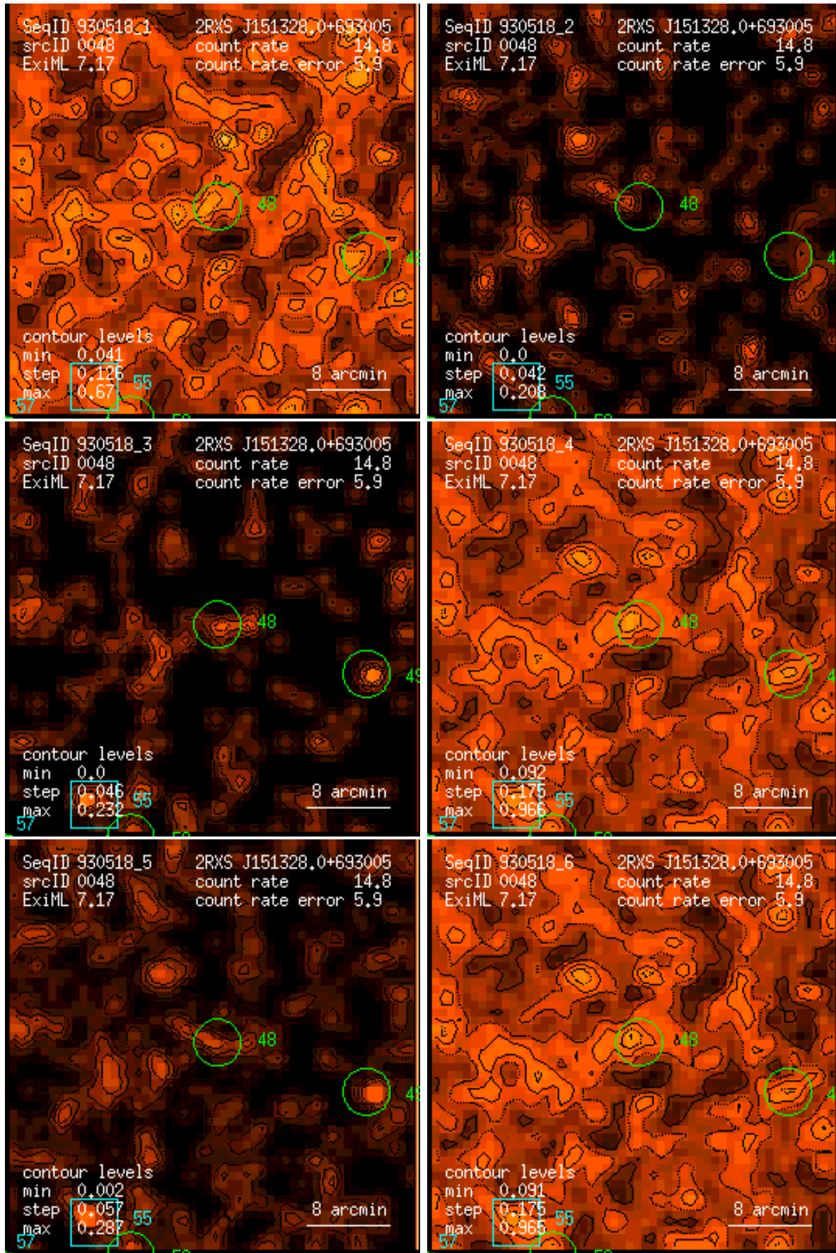
Figure 48: RASS 930518: detection 0048: band rate images, Gaussian filter: (1) PSPC channels 11 – 41, (2) 52 – 90, (3) 91 – 201, (4) 11 – 235, (5) 52 – 201, (6) 11 – 201. Broad band rates in counts/ks. Band rate contour levels in counts/ks/arcmin 2 .
