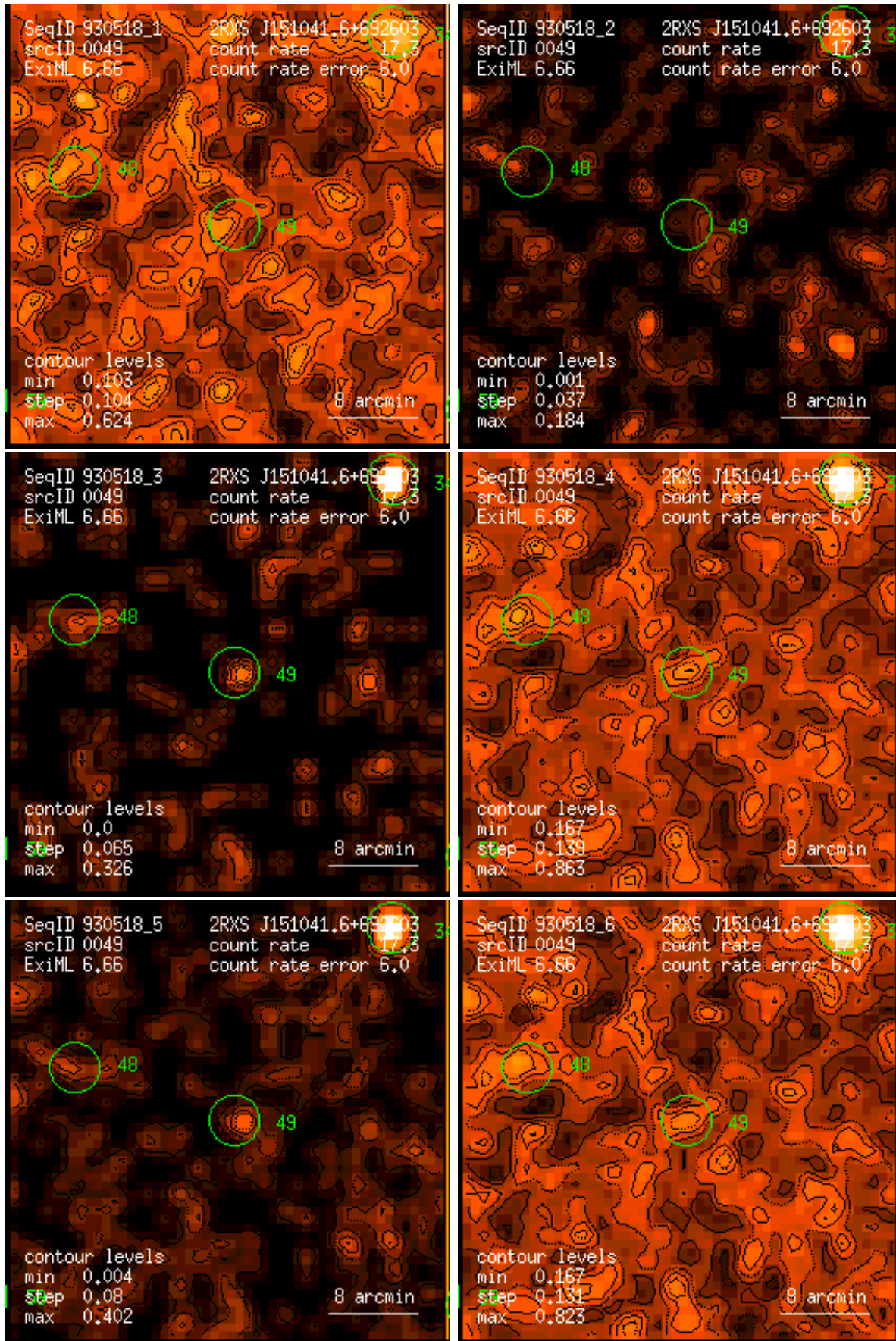
Figure 49: RASS 930518: detection 0049: band rate images, Gaussian filter: (1) PSPC channels 11 – 41, (2) 52 – 90, (3) 91 – 201, (4) 11 – 235, (5) 52 – 201, (6) 11 – 201. Broad band rates in counts/ks. Band rate contour levels in counts/ks/arcmin 2 .
