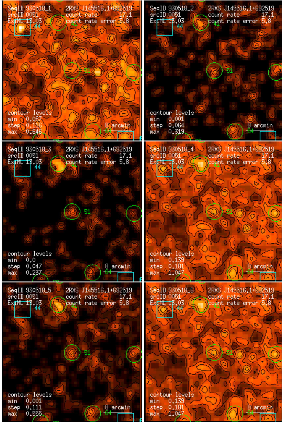
Figure 51: RASS 930518: detection 0051: band rate images, Gaussian filter: (1) PSPC channels 11 – 41, (2) 52 – 90, (3) 91 – 201, (4) 11 – 235, (5) 52 – 201, (6) 11 – 201. Broad band rates in counts/ks. Band rate contour levels in counts/ks/arcmin 2 .
