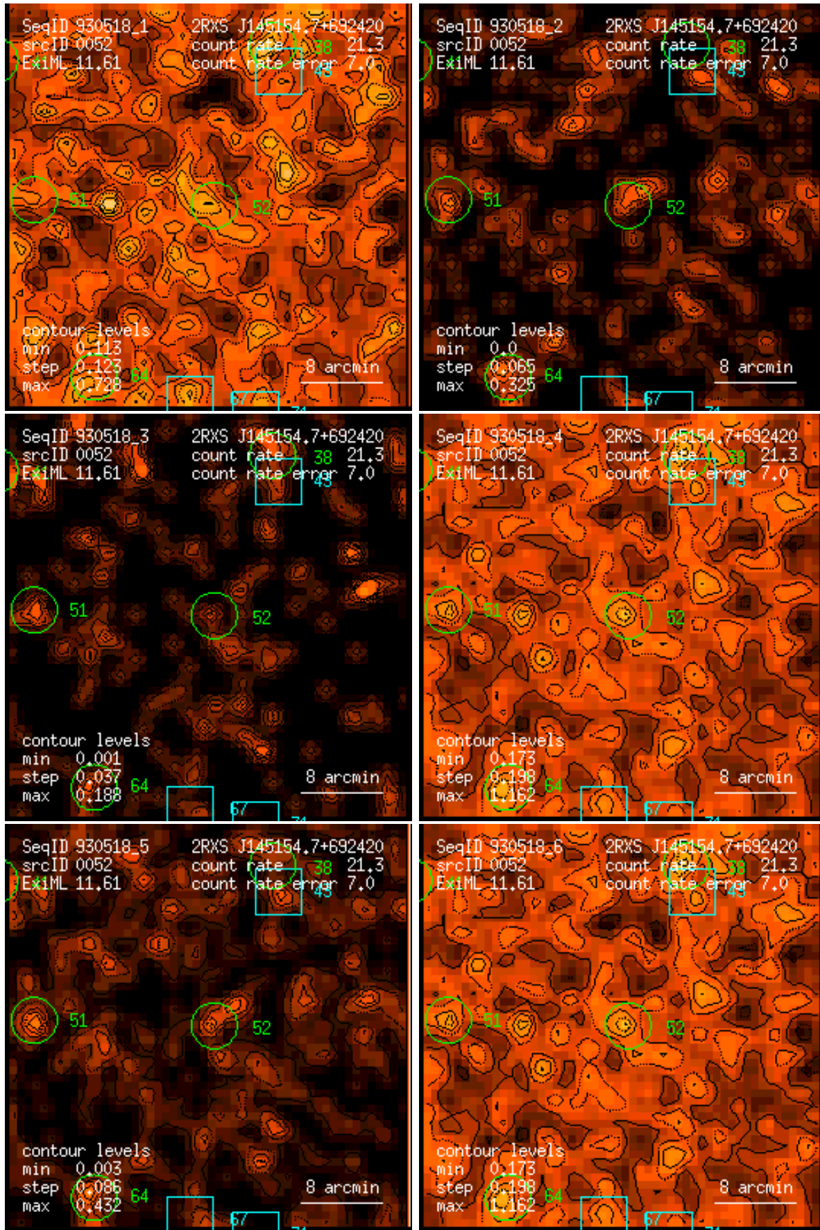
Figure 52: RASS 930518: detection 0052: band rate images, Gaussian filter: (1) PSPC channels 11 – 41, (2) 52 – 90, (3) 91 – 201, (4) 11 – 235, (5) 52 – 201, (6) 11 – 201. Broad band rates in counts/ks. Band rate contour levels in counts/ks/arcmin 2 .
