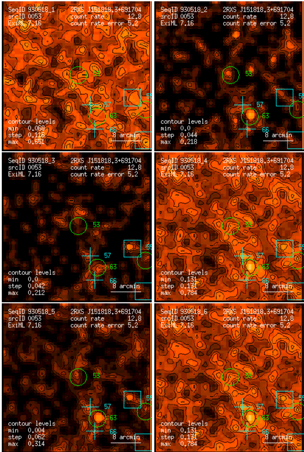
Figure 53: RASS 930518: detection 0053: band rate images, Gaussian filter: (1) PSPC channels 11 – 41, (2) 52 – 90, (3) 91 – 201, (4) 11 – 235, (5) 52 – 201, (6) 11 – 201. Broad band rates in counts/ks. Band rate contour levels in counts/ks/arcmin 2 .
