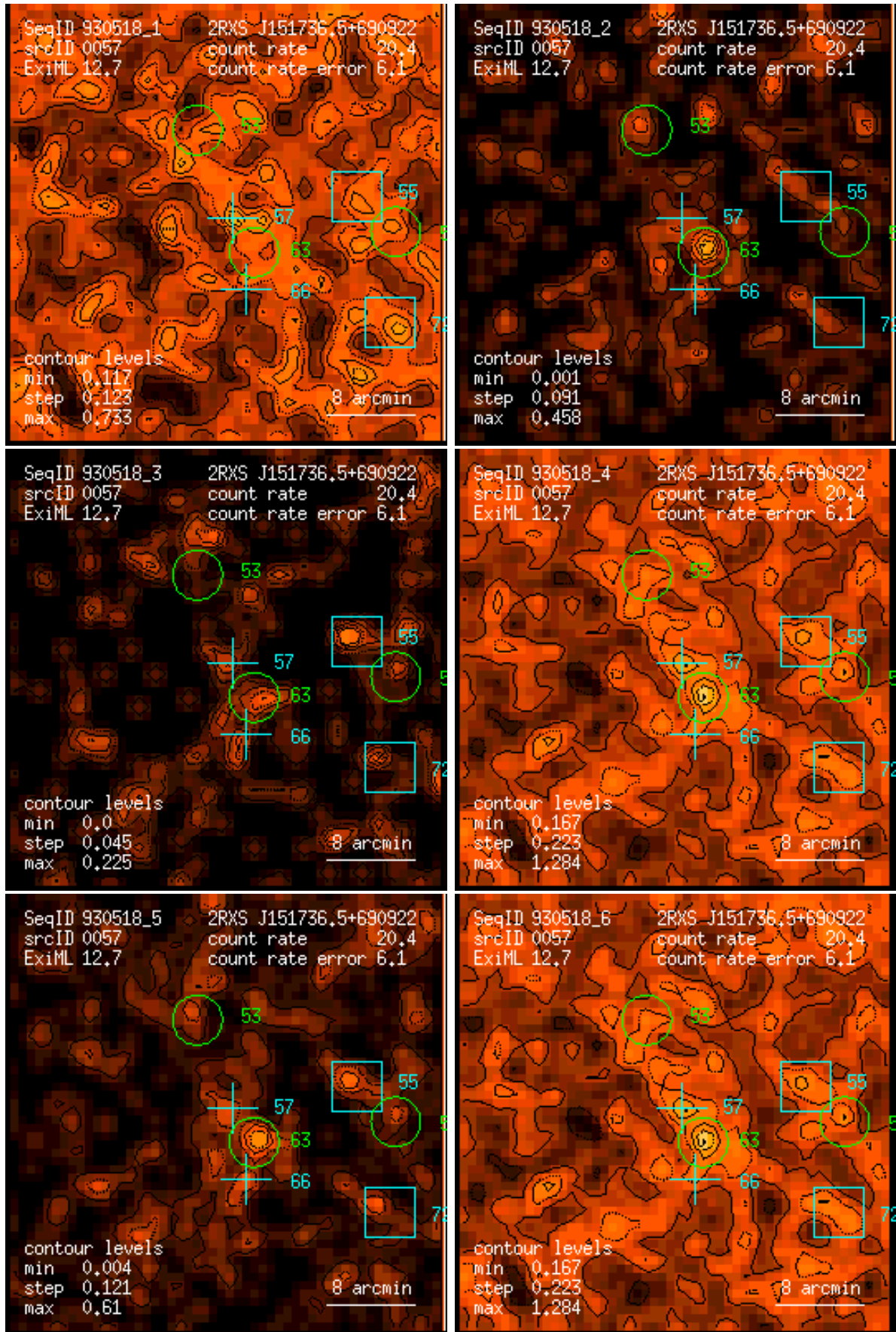
Figure 57: RASS 930518: detection 0057: band rate images, Gaussian filter: (1) PSPC channels 11 – 41, (2) 52 – 90, (3) 91 – 201, (4) 11 – 235, (5) 52 – 201, (6) 11 – 201. Broad band rates in counts/ks. Band rate contour levels in counts/ks/arcmin 2 .
