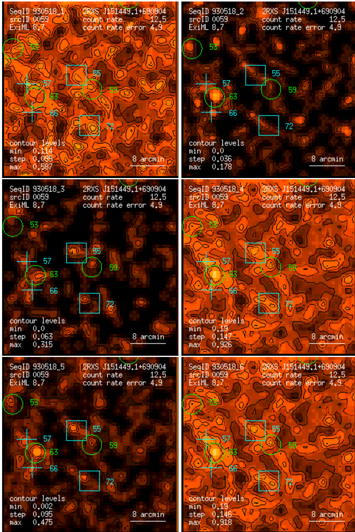
Figure 59: RASS 930518: detection 0059: band rate images, Gaussian filter: (1) PSPC channels 11 – 41, (2) 52 – 90, (3) 91 – 201, (4) 11 – 235, (5) 52 – 201, (6) 11 – 201. Broad band rates in counts/ks. Band rate contour levels in counts/ks/arcmin 2 .
