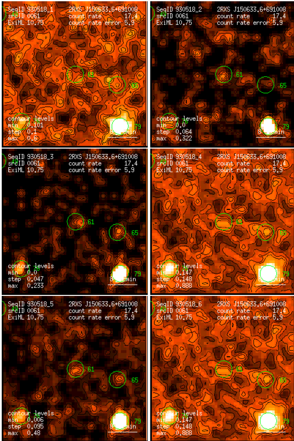
Figure 61: RASS 930518: detection 0061: band rate images, Gaussian filter: (1) PSPC channels 11 – 41, (2) 52 – 90, (3) 91 – 201, (4) 11 – 235, (5) 52 – 201, (6) 11 – 201. Broad band rates in counts/ks. Band rate contour levels in counts/ks/arcmin 2 .
