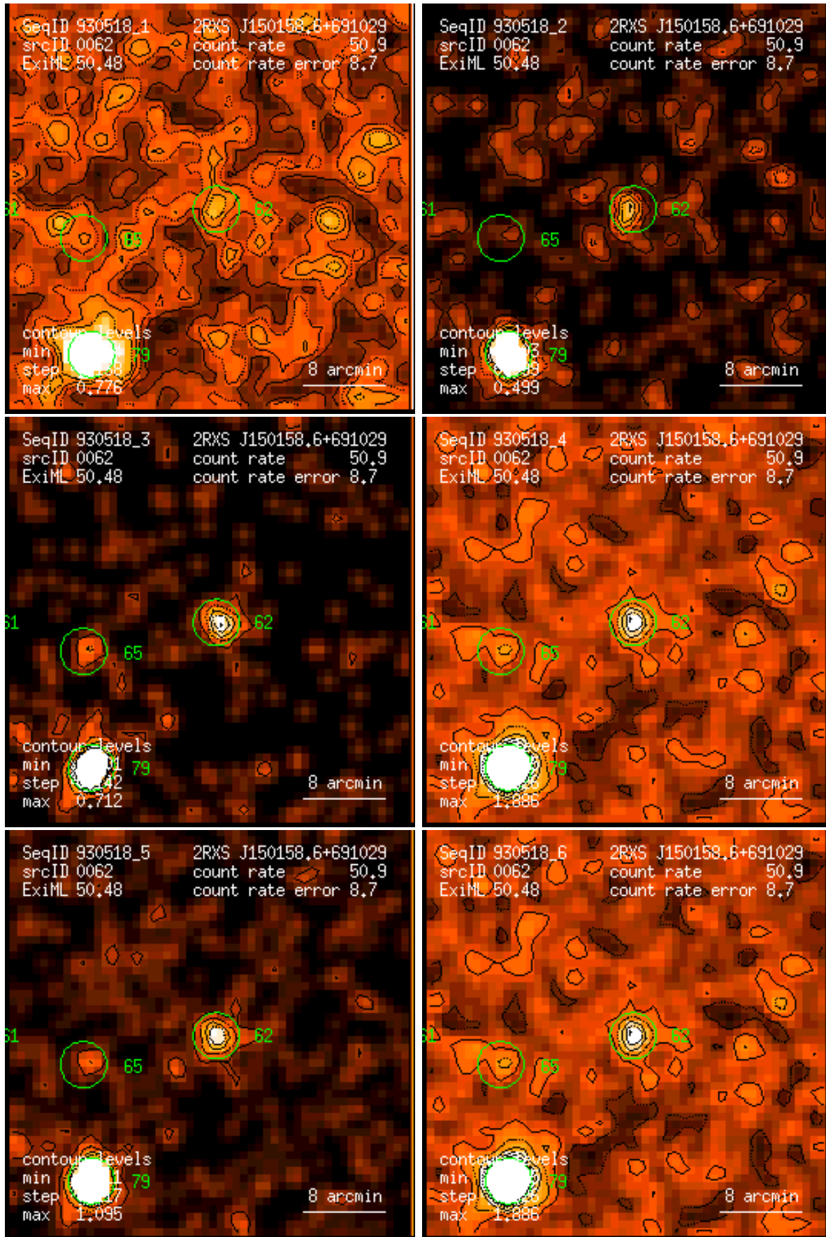
Figure 62: RASS 930518: detection 0062: band rate images, Gaussian filter: (1) PSPC channels 11 – 41, (2) 52 – 90, (3) 91 – 201, (4) 11 – 235, (5) 52 – 201, (6) 11 – 201. Broad band rates in counts/ks. Band rate contour levels in counts/ks/arcmin 2 .
