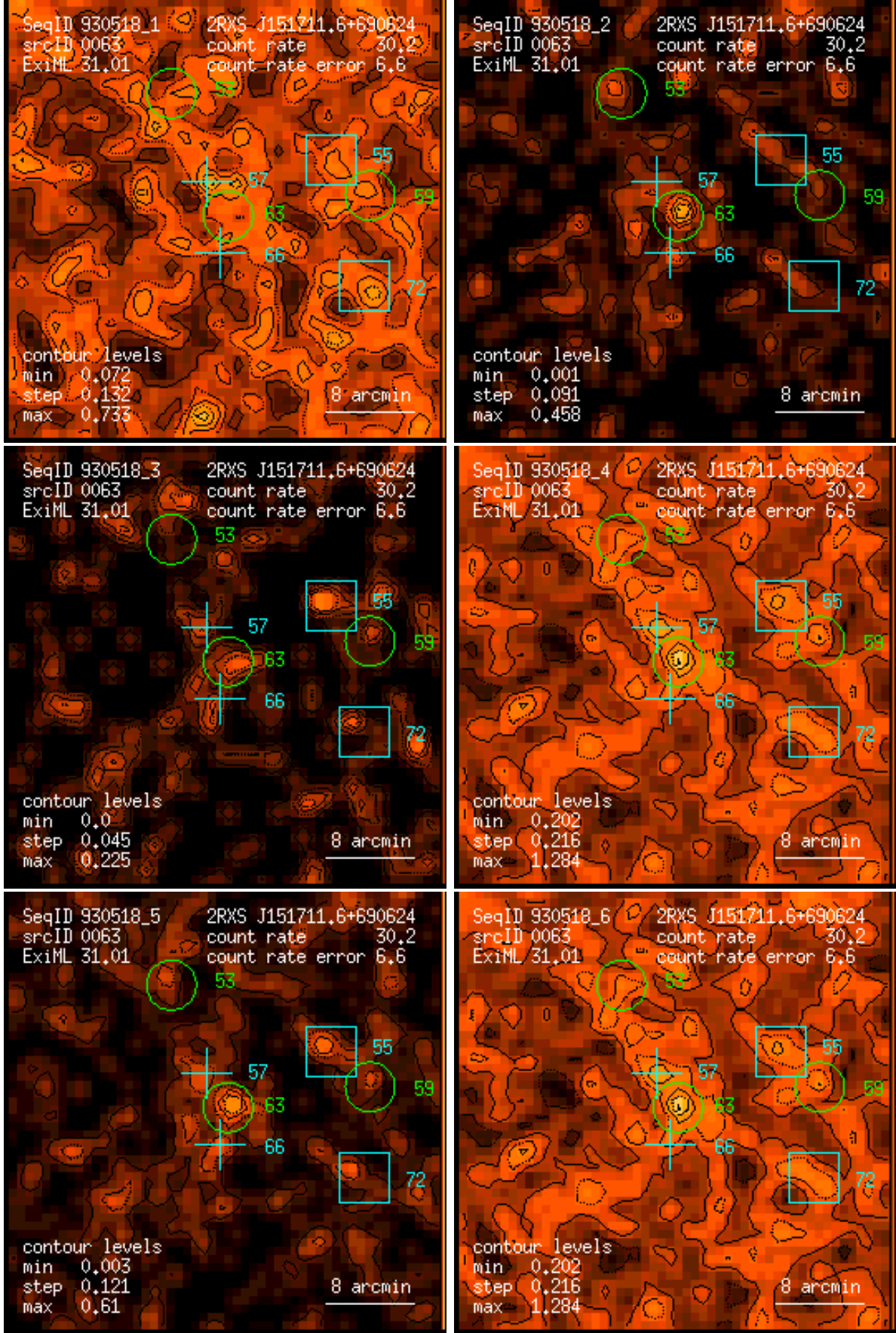
Figure 63: RASS 930518: detection 0063: band rate images, Gaussian filter: (1) PSPC channels 11 – 41, (2) 52 – 90, (3) 91 – 201, (4) 11 – 235, (5) 52 – 201, (6) 11 – 201. Broad band rates in counts/ks. Band rate contour levels in counts/ks/arcmin 2 .
