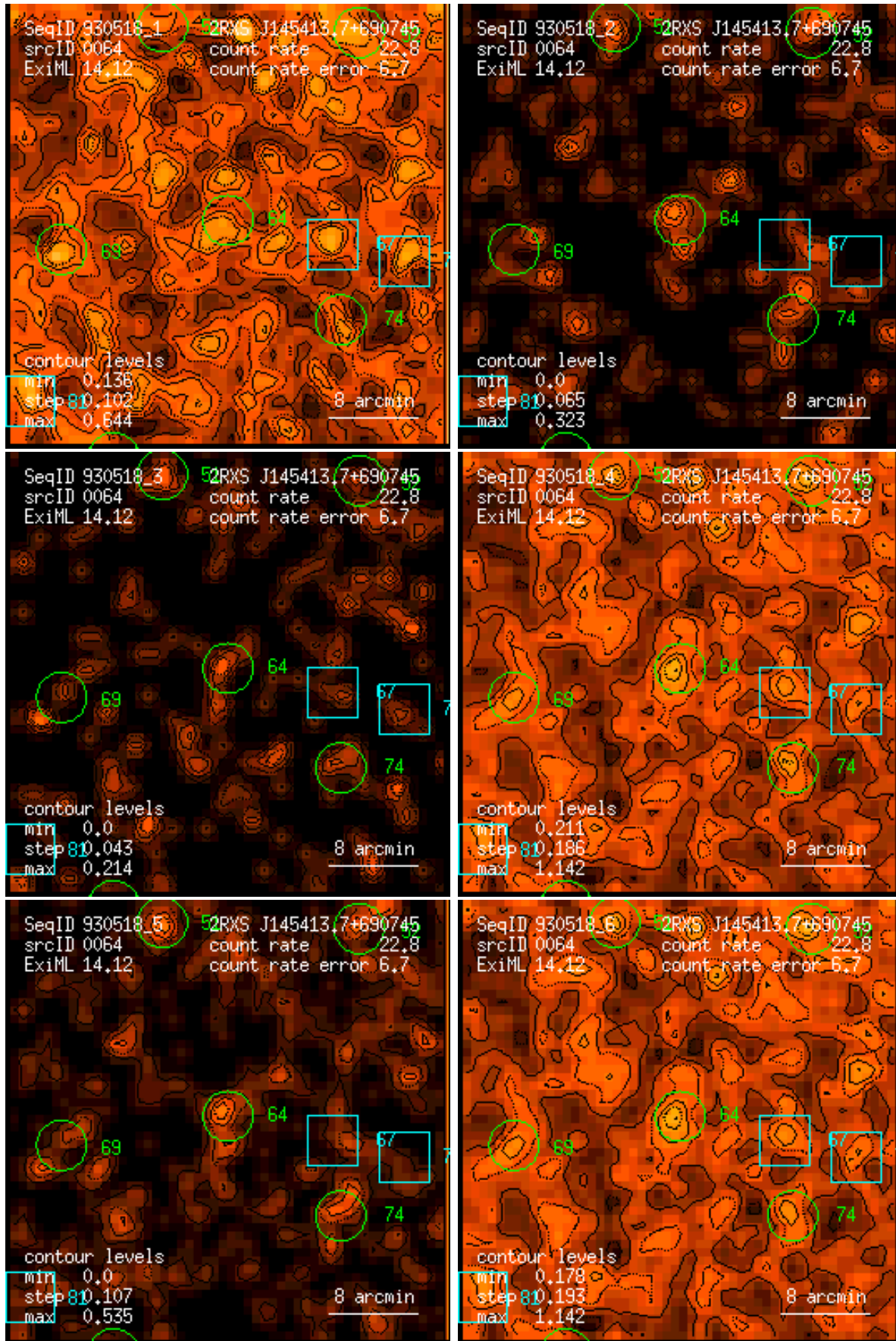
Figure 64: RASS 930518: detection 0064: band rate images, Gaussian filter: (1) PSPC channels 11 – 41, (2) 52 – 90, (3) 91 – 201, (4) 11 – 235, (5) 52 – 201, (6) 11 – 201. Broad band rates in counts/ks. Band rate contour levels in counts/ks/arcmin 2 .
