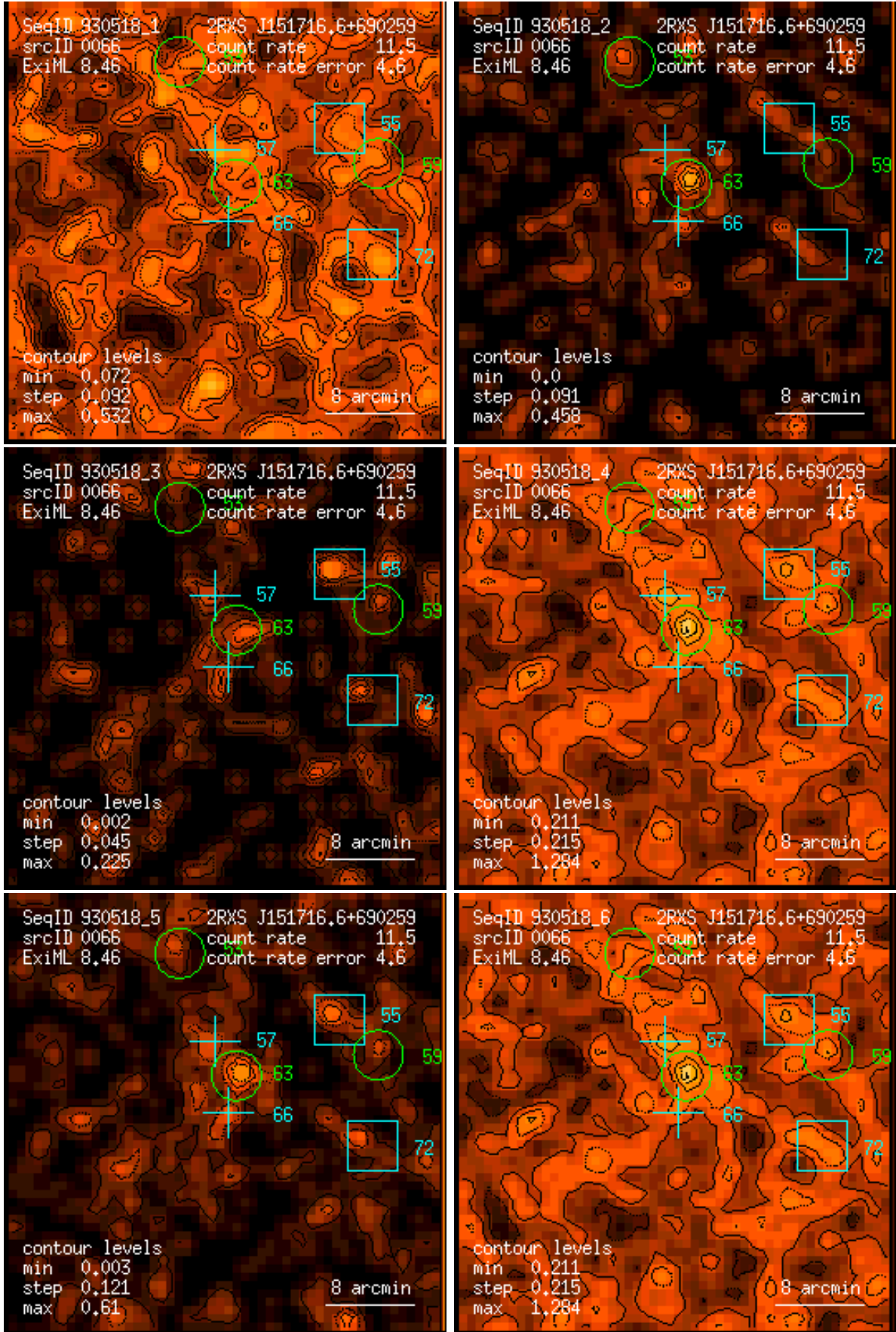
Figure 66: RASS 930518: detection 0066: band rate images, Gaussian filter: (1) PSPC channels 11 – 41, (2) 52 – 90, (3) 91 – 201, (4) 11 – 235, (5) 52 – 201, (6) 11 – 201. Broad band rates in counts/ks. Band rate contour levels in counts/ks/arcmin 2 .
