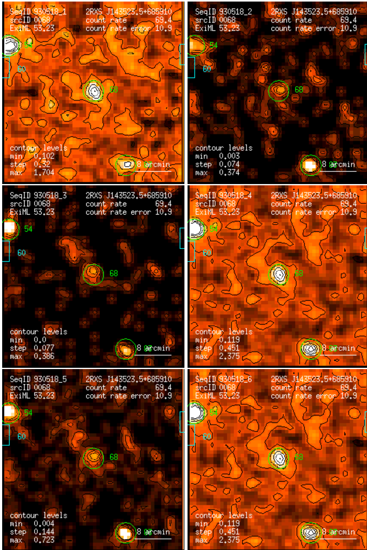
Figure 68: RASS 930518: detection 0068: band rate images, Gaussian filter: (1) PSPC channels 11 – 41, (2) 52 – 90, (3) 91 – 201, (4) 11 – 235, (5) 52 – 201, (6) 11 – 201. Broad band rates in counts/ks. Band rate contour levels in counts/ks/arcmin 2 .
