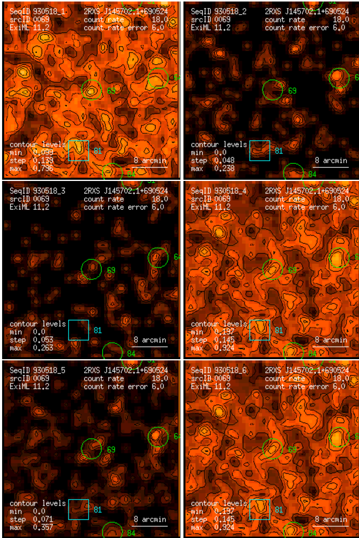
Figure 69: RASS 930518: detection 0069: band rate images, Gaussian filter: (1) PSPC channels 11 – 41, (2) 52 – 90, (3) 91 – 201, (4) 11 – 235, (5) 52 – 201, (6) 11 – 201. Broad band rates in counts/ks. Band rate contour levels in counts/ks/arcmin 2 .
