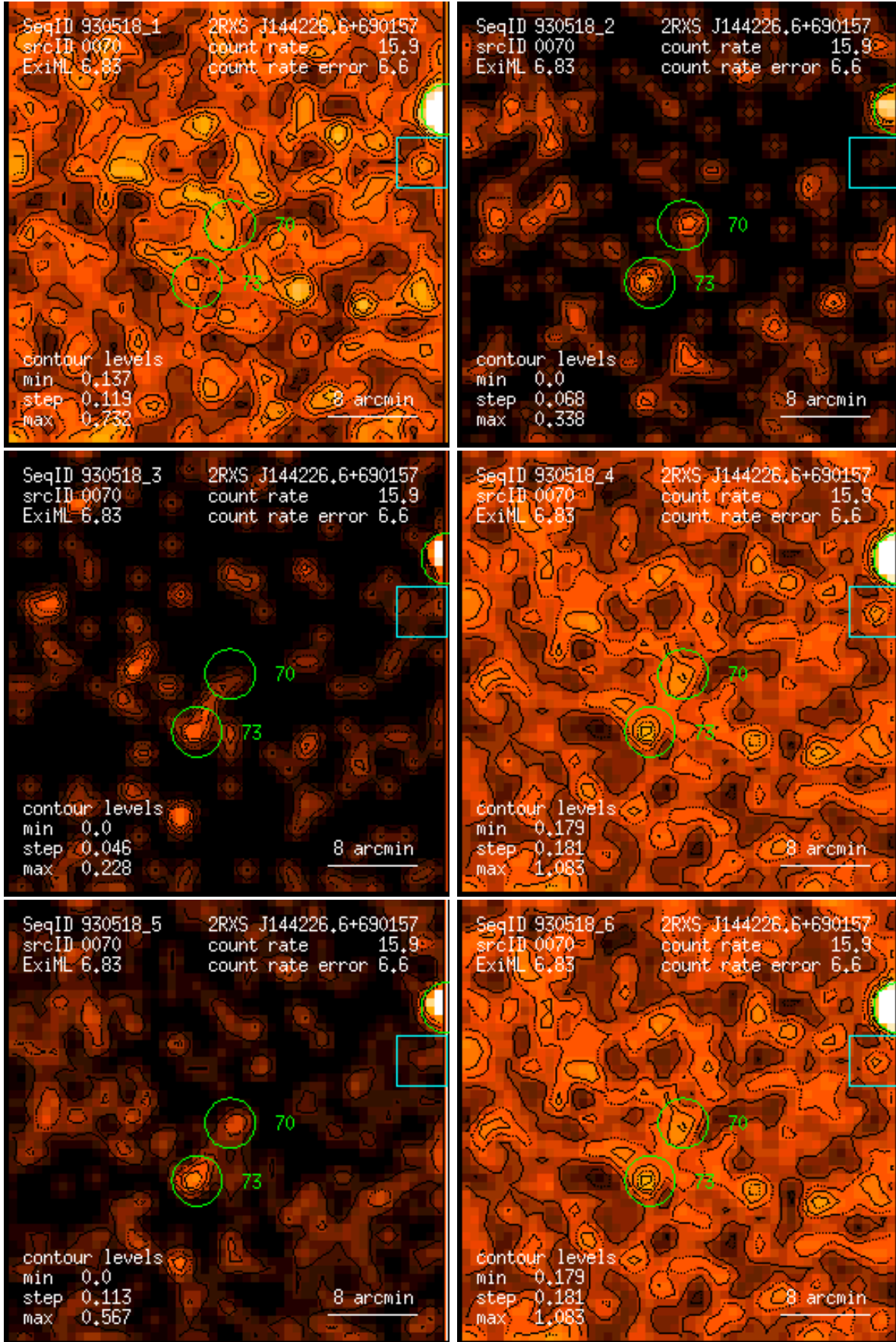
Figure 70: RASS 930518: detection 0070: band rate images, Gaussian filter: (1) PSPC channels 11 – 41, (2) 52 – 90, (3) 91 – 201, (4) 11 – 235, (5) 52 – 201, (6) 11 – 201. Broad band rates in counts/ks. Band rate contour levels in counts/ks/arcmin 2 .
