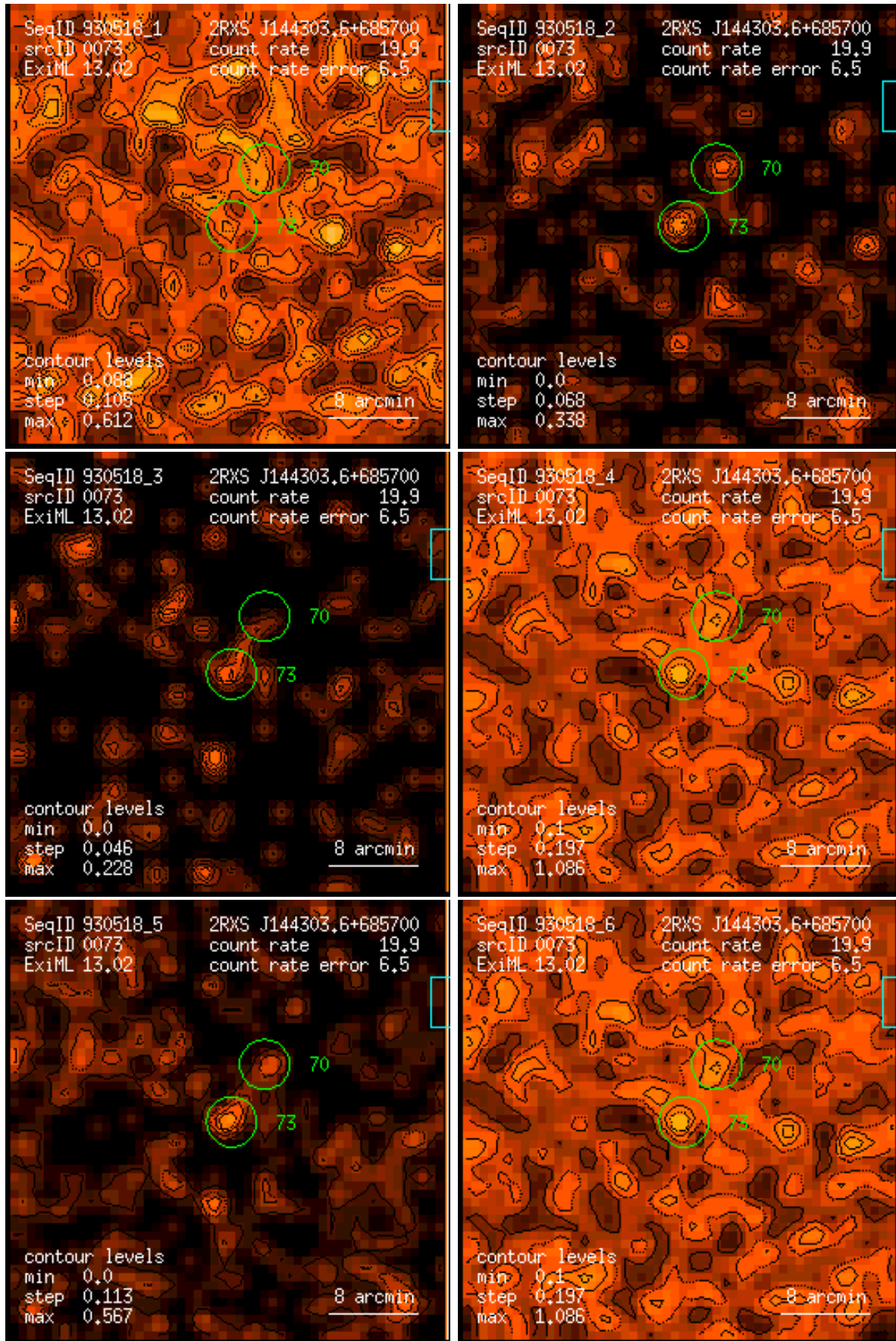
Figure 73: RASS 930518: detection 0073: band rate images, Gaussian filter: (1) PSPC channels 11 – 41, (2) 52 – 90, (3) 91 – 201, (4) 11 – 235, (5) 52 – 201, (6) 11 – 201. Broad band rates in counts/ks. Band rate contour levels in counts/ks/arcmin 2 .
