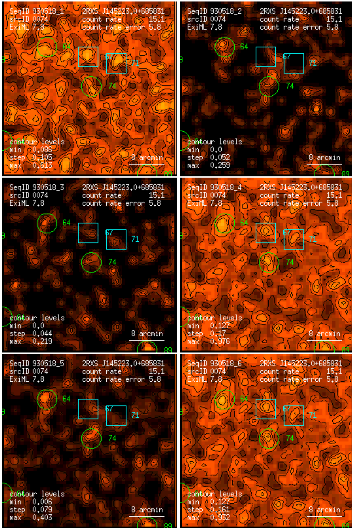
Figure 74: RASS 930518: detection 0074: band rate images, Gaussian filter: (1) PSPC channels 11 – 41, (2) 52 – 90, (3) 91 – 201, (4) 11 – 235, (5) 52 – 201, (6) 11 – 201. Broad band rates in counts/ks. Band rate contour levels in counts/ks/arcmin 2 .
