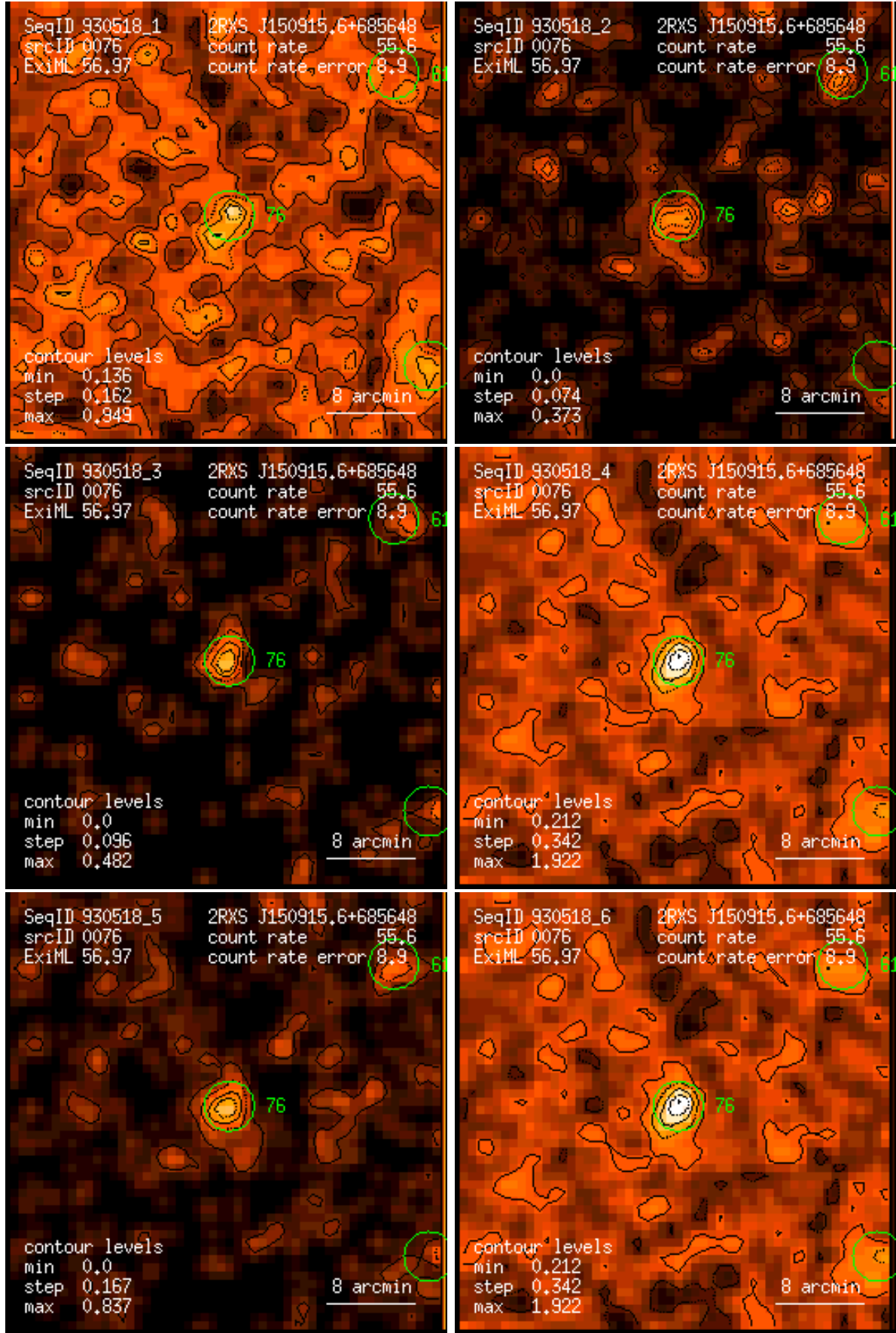
Figure 76: RASS 930518: detection 0076: band rate images, Gaussian filter: (1) PSPC channels 11 – 41, (2) 52 – 90, (3) 91 – 201, (4) 11 – 235, (5) 52 – 201, (6) 11 – 201. Broad band rates in counts/ks. Band rate contour levels in counts/ks/arcmin 2 .
