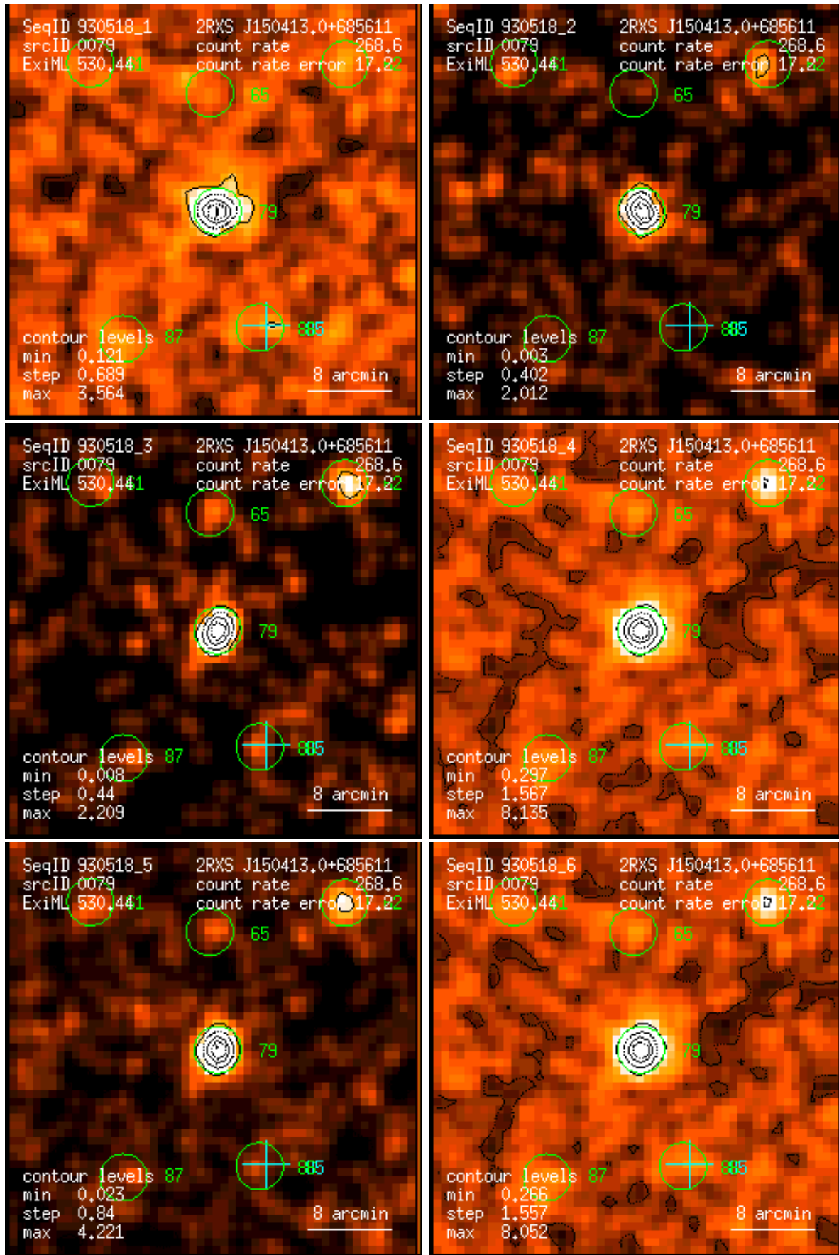
Figure 79: RASS 930518: detection 0079: band rate images, Gaussian filter: (1) PSPC channels 11 – 41, (2) 52 – 90, (3) 91 – 201, (4) 11 – 235, (5) 52 – 201, (6) 11 – 201. Broad band rates in counts/ks. Band rate contour levels in counts/ks/arcmin 2 .
