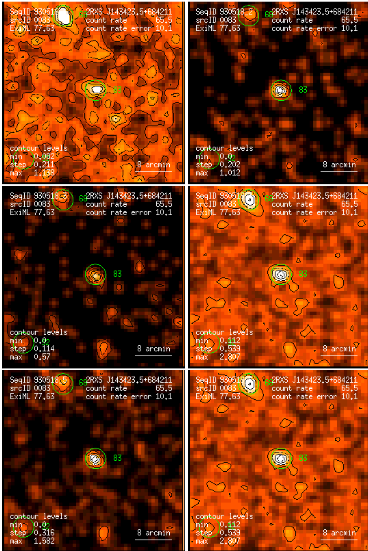
Figure 83: RASS 930518: detection 0083: band rate images, Gaussian filter: (1) PSPC channels 11 – 41, (2) 52 – 90, (3) 91 – 201, (4) 11 – 235, (5) 52 – 201, (6) 11 – 201. Broad band rates in counts/ks. Band rate contour levels in counts/ks/arcmin 2 .
