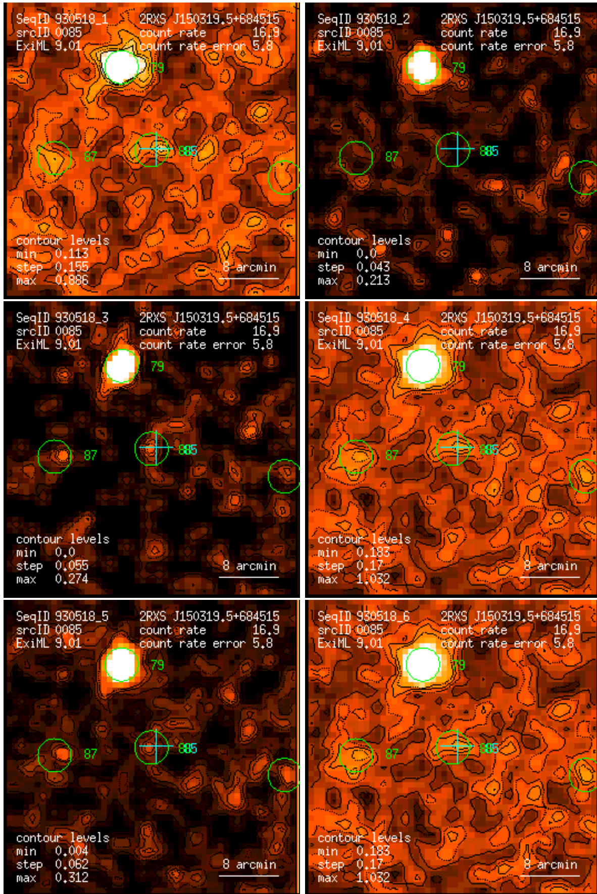
Figure 85: RASS 930518: detection 0085: band rate images, Gaussian filter: (1) PSPC channels 11 – 41, (2) 52 – 90, (3) 91 – 201, (4) 11 – 235, (5) 52 – 201, (6) 11 – 201. Broad band rates in counts/ks. Band rate contour levels in counts/ks/arcmin 2 .
