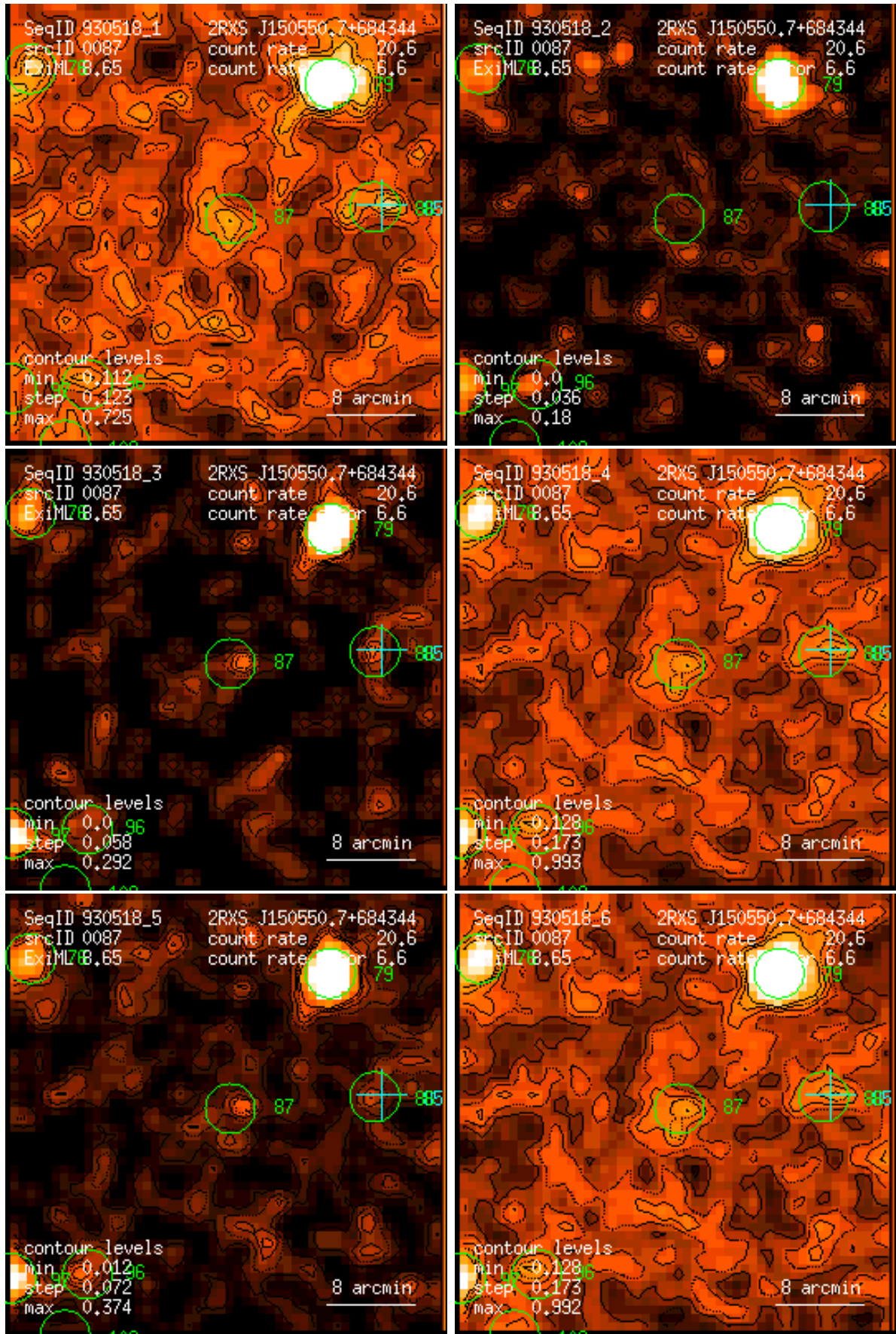
Figure 87: RASS 930518: detection 0087: band rate images, Gaussian filter: (1) PSPC channels 11 – 41, (2) 52 – 90, (3) 91 – 201, (4) 11 – 235, (5) 52 – 201, (6) 11 – 201. Broad band rates in counts/ks. Band rate contour levels in counts/ks/arcmin 2 .
