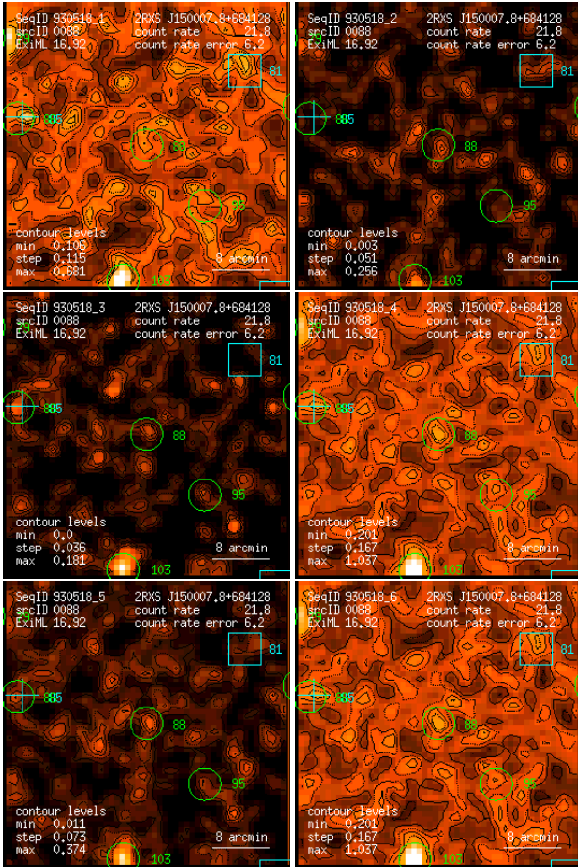
Figure 88: RASS 930518: detection 0088: band rate images, Gaussian filter: (1) PSPC channels 11 – 41, (2) 52 – 90, (3) 91 – 201, (4) 11 – 235, (5) 52 – 201, (6) 11 – 201. Broad band rates in counts/ks. Band rate contour levels in counts/ks/arcmin 2 .
