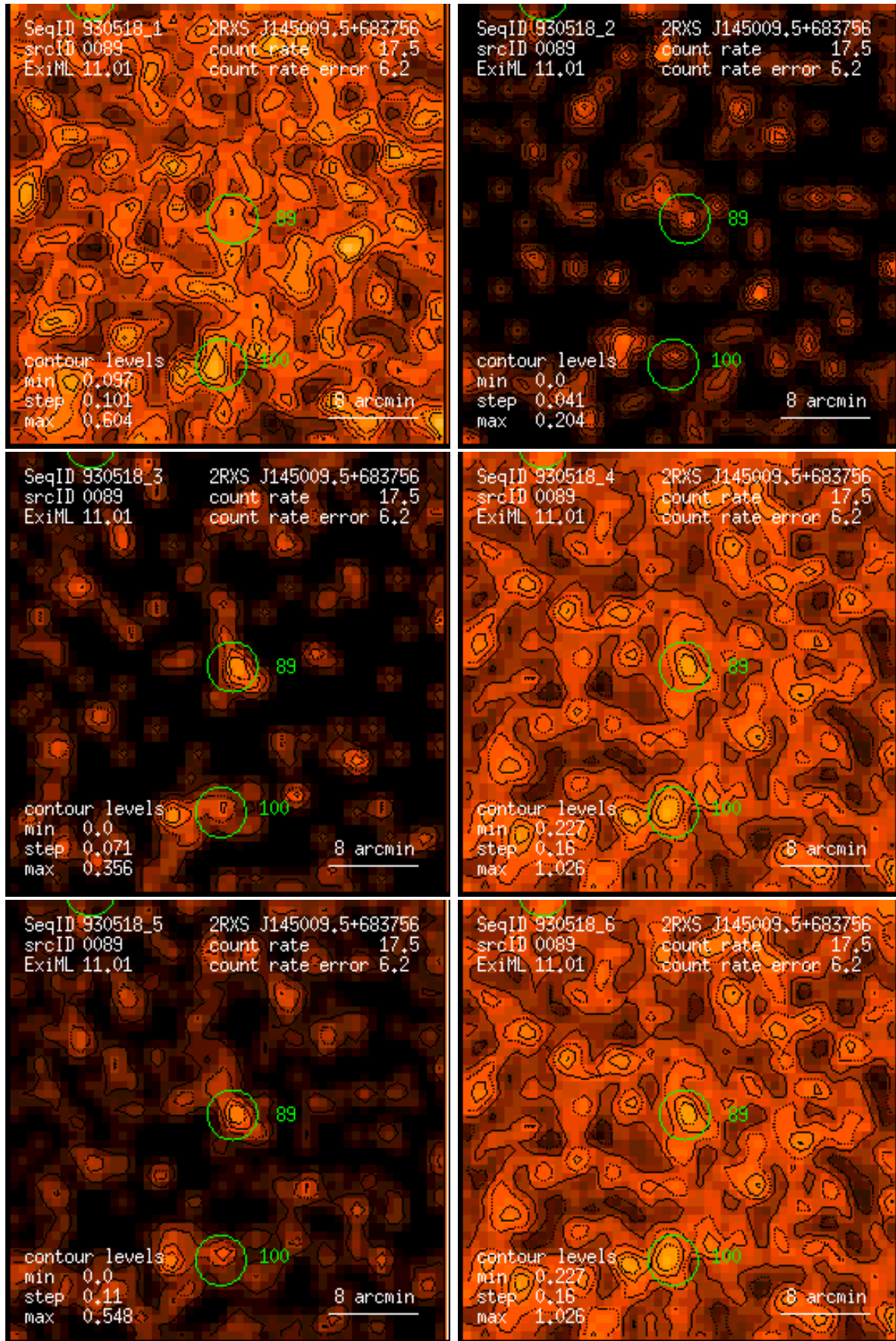
Figure 89: RASS 930518: detection 0089: band rate images, Gaussian filter: (1) PSPC channels 11 – 41, (2) 52 – 90, (3) 91 – 201, (4) 11 – 235, (5) 52 – 201, (6) 11 – 201. Broad band rates in counts/ks. Band rate contour levels in counts/ks/arcmin 2 .
