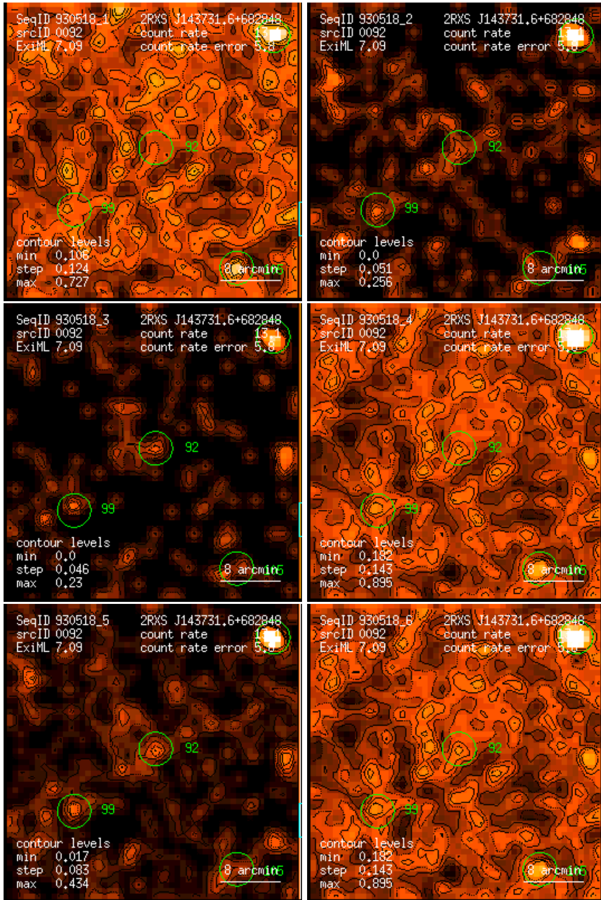
Figure 92: RASS 930518: detection 0092: band rate images, Gaussian filter: (1) PSPC channels 11 – 41, (2) 52 – 90, (3) 91 – 201, (4) 11 – 235, (5) 52 – 201, (6) 11 – 201. Broad band rates in counts/ks. Band rate contour levels in counts/ks/arcmin 2 .
