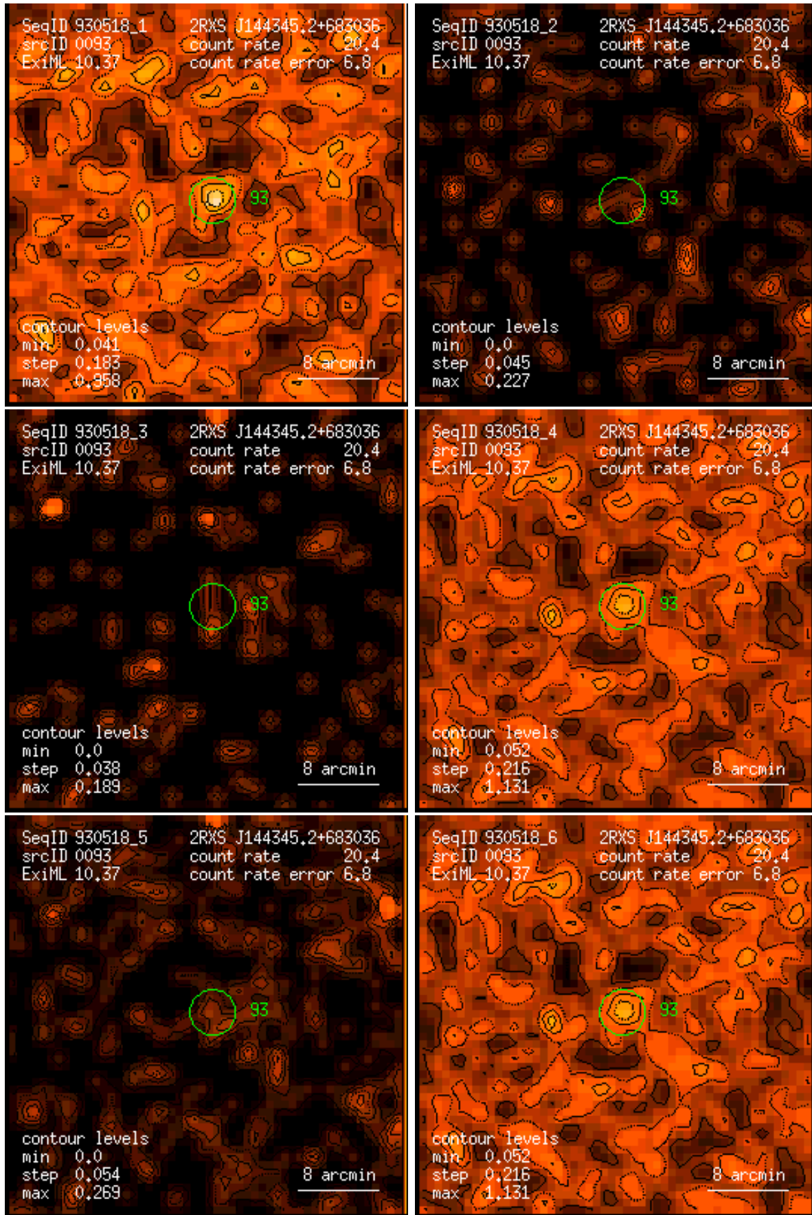
Figure 93: RASS 930518: detection 0093: band rate images, Gaussian filter: (1) PSPC channels 11 – 41, (2) 52 – 90, (3) 91 – 201, (4) 11 – 235, (5) 52 – 201, (6) 11 – 201. Broad band rates in counts/ks. Band rate contour levels in counts/ks/arcmin 2 .
