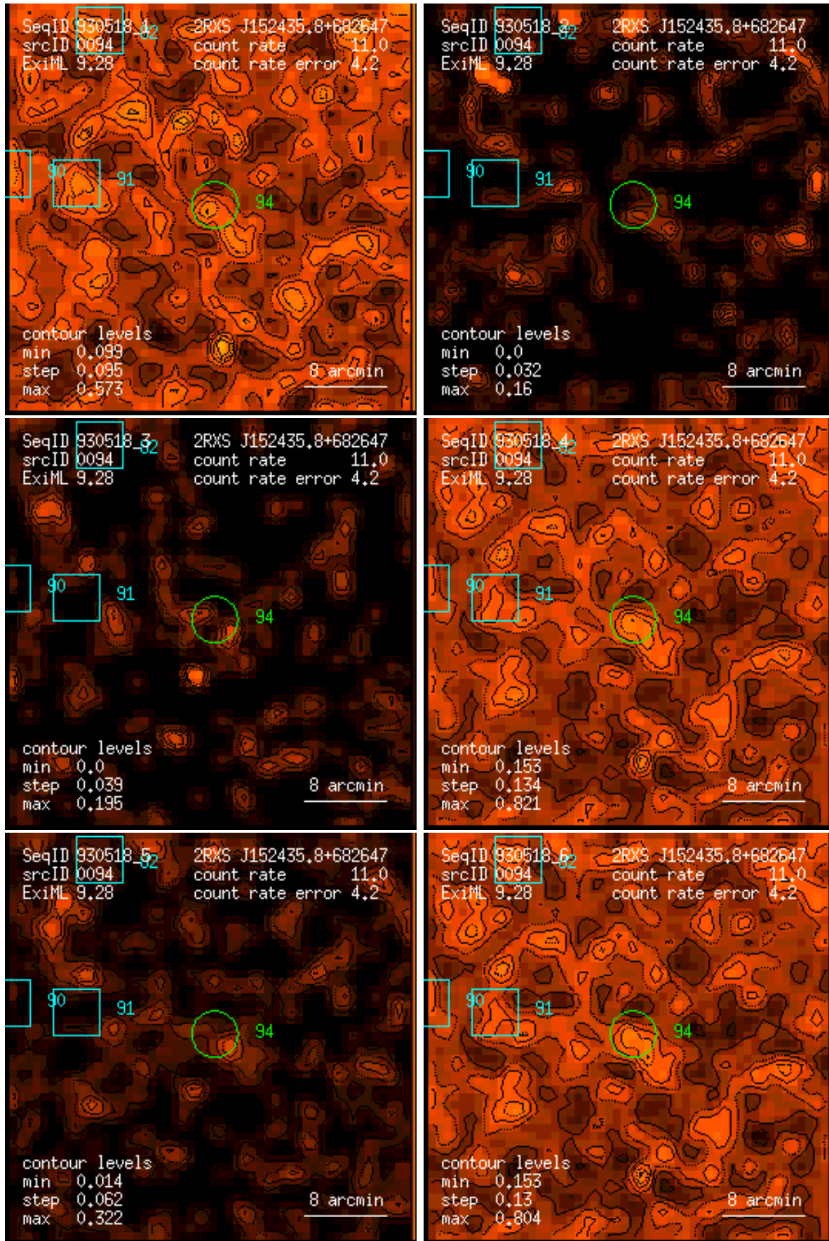
Figure 94: RASS 930518: detection 0094: band rate images, Gaussian filter: (1) PSPC channels 11 – 41, (2) 52 – 90, (3) 91 – 201, (4) 11 – 235, (5) 52 – 201, (6) 11 – 201. Broad band rates in counts/ks. Band rate contour levels in counts/ks/arcmin 2 .
