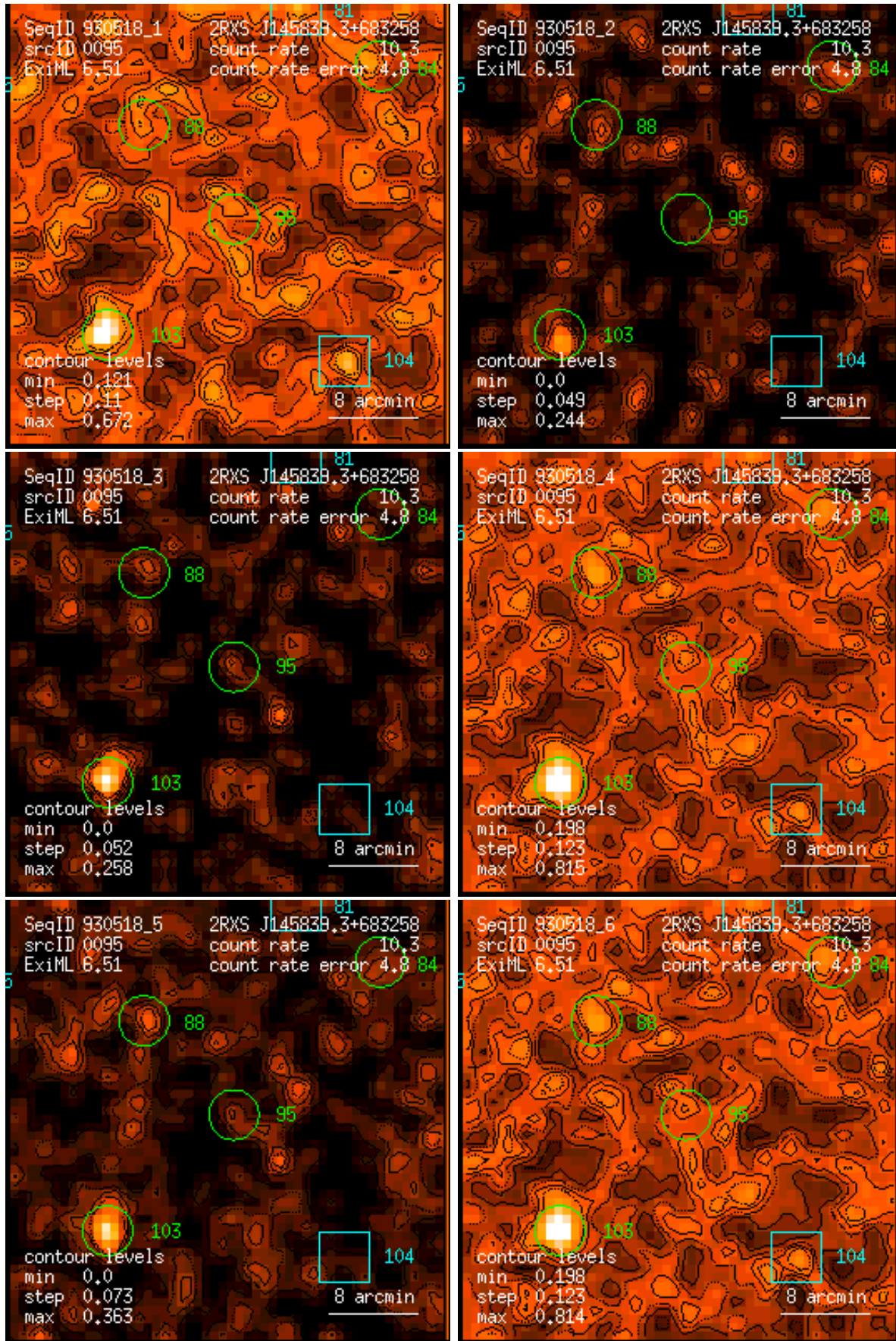
Figure 95: RASS 930518: detection 0095: band rate images, Gaussian filter: (1) PSPC channels 11 – 41, (2) 52 – 90, (3) 91 – 201, (4) 11 – 235, (5) 52 – 201, (6) 11 – 201. Broad band rates in counts/ks. Band rate contour levels in counts/ks/arcmin 2 .
