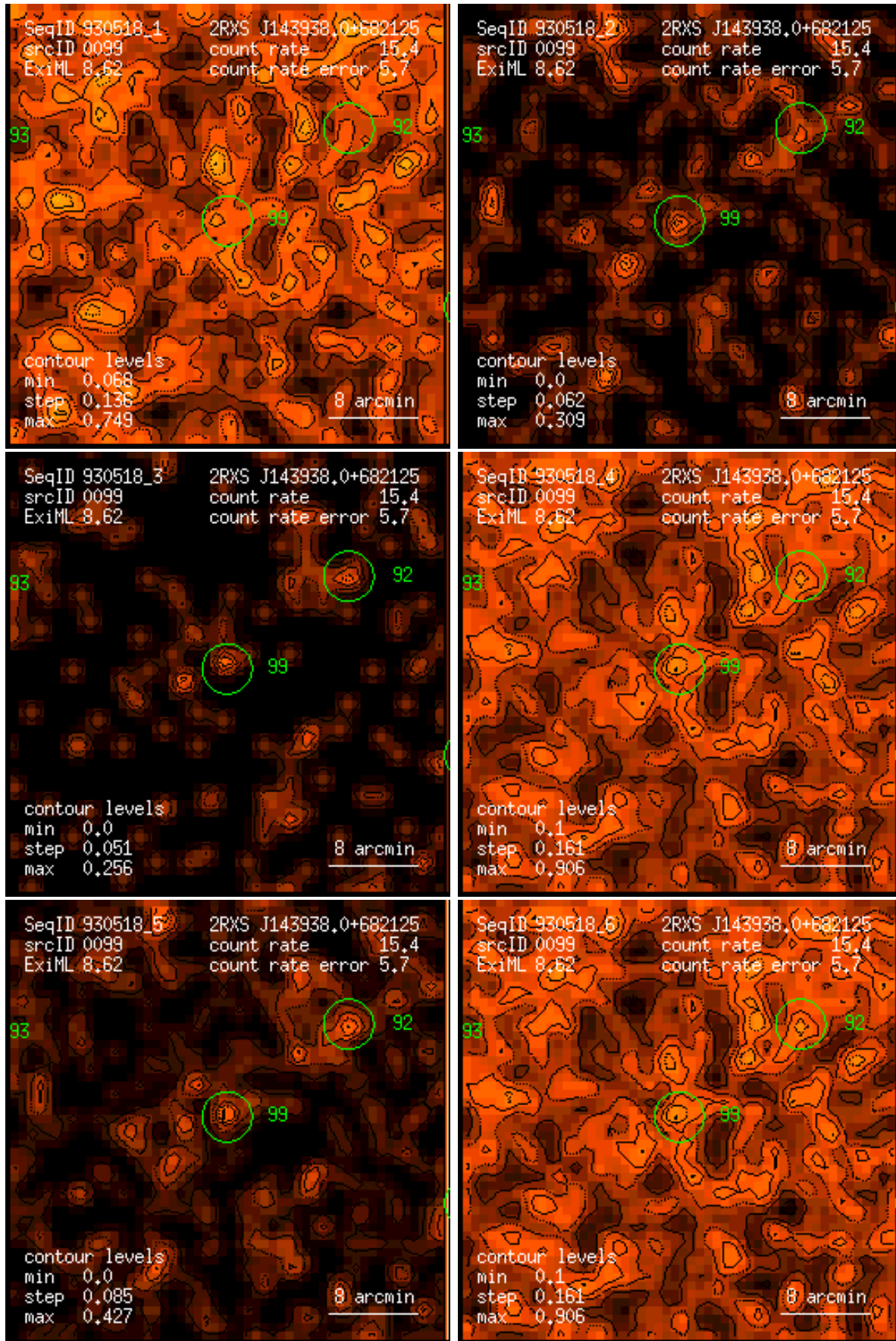
Figure 99: RASS 930518: detection 0099: band rate images, Gaussian filter: (1) PSPC channels 11 – 41, (2) 52 – 90, (3) 91 – 201, (4) 11 – 235, (5) 52 – 201, (6) 11 – 201. Broad band rates in counts/ks. Band rate contour levels in counts/ks/arcmin 2 .
