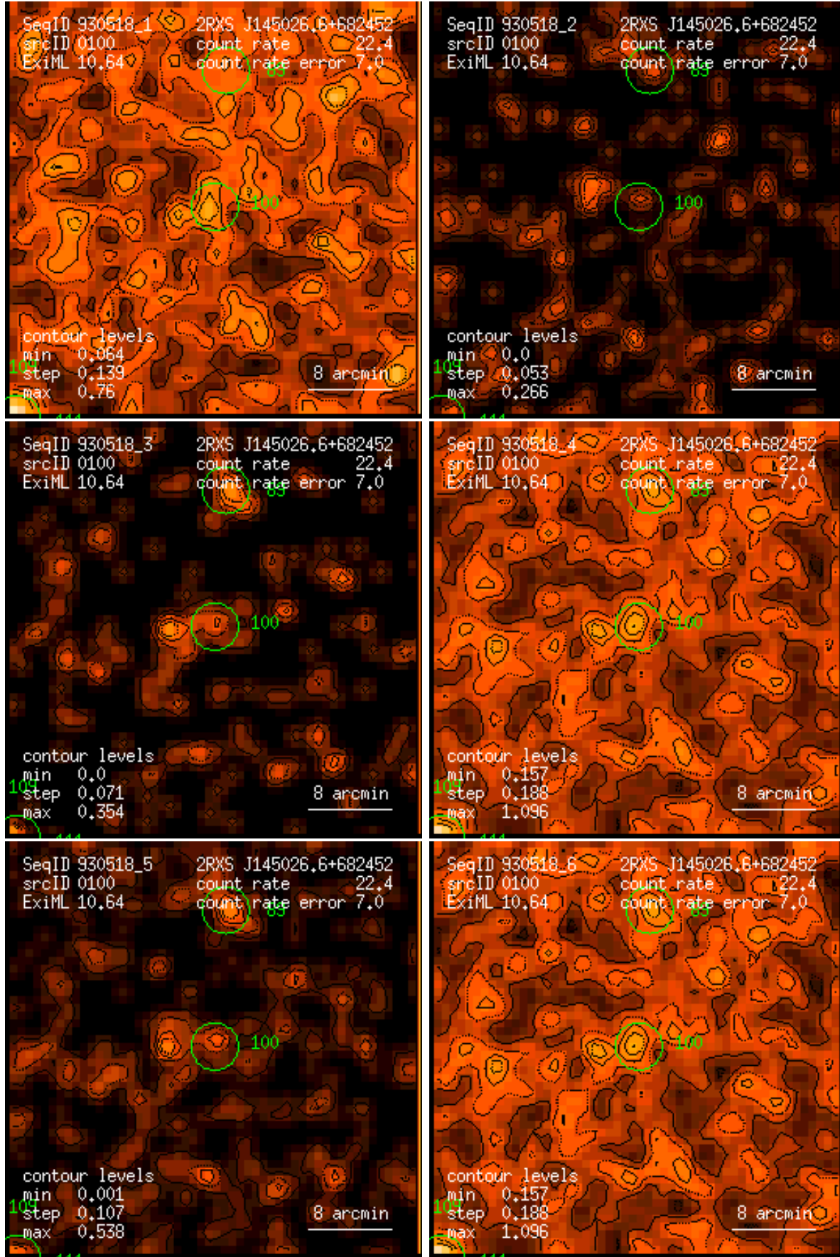
Figure 100: RASS 930518: detection 0100: band rate images, Gaussian filter: (1) PSPC channels 11 – 41, (2) 52 – 90, (3) 91 – 201, (4) 11 – 235, (5) 52 – 201, (6) 11 – 201. Broad band rates in counts/ks. Band rate contour levels in counts/ks/arcmin 2 .
