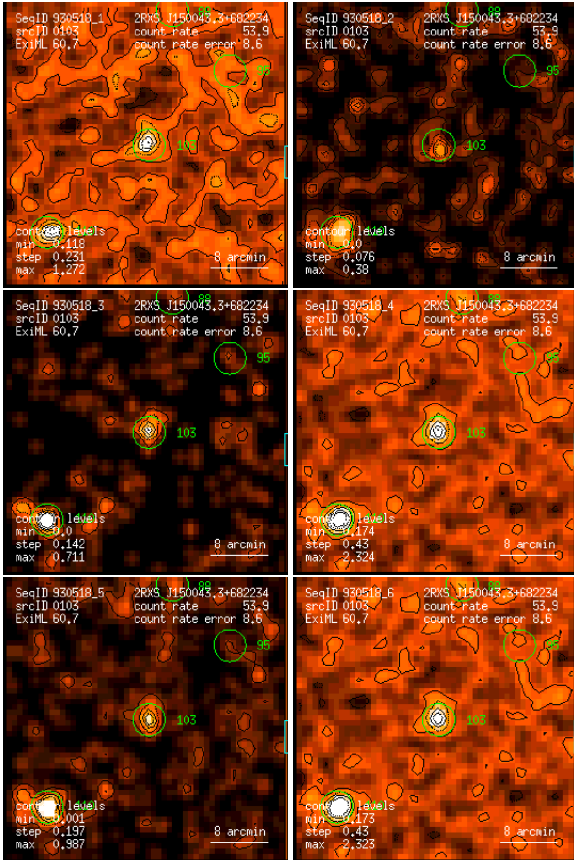
Figure 103: RASS 930518: detection 0103: band rate images, Gaussian filter: (1) PSPC channels 11 – 41, (2) 52 – 90, (3) 91 – 201, (4) 11 – 235, (5) 52 – 201, (6) 11 – 201. Broad band rates in counts/ks. Band rate contour levels in counts/ks/arcmin 2 .
