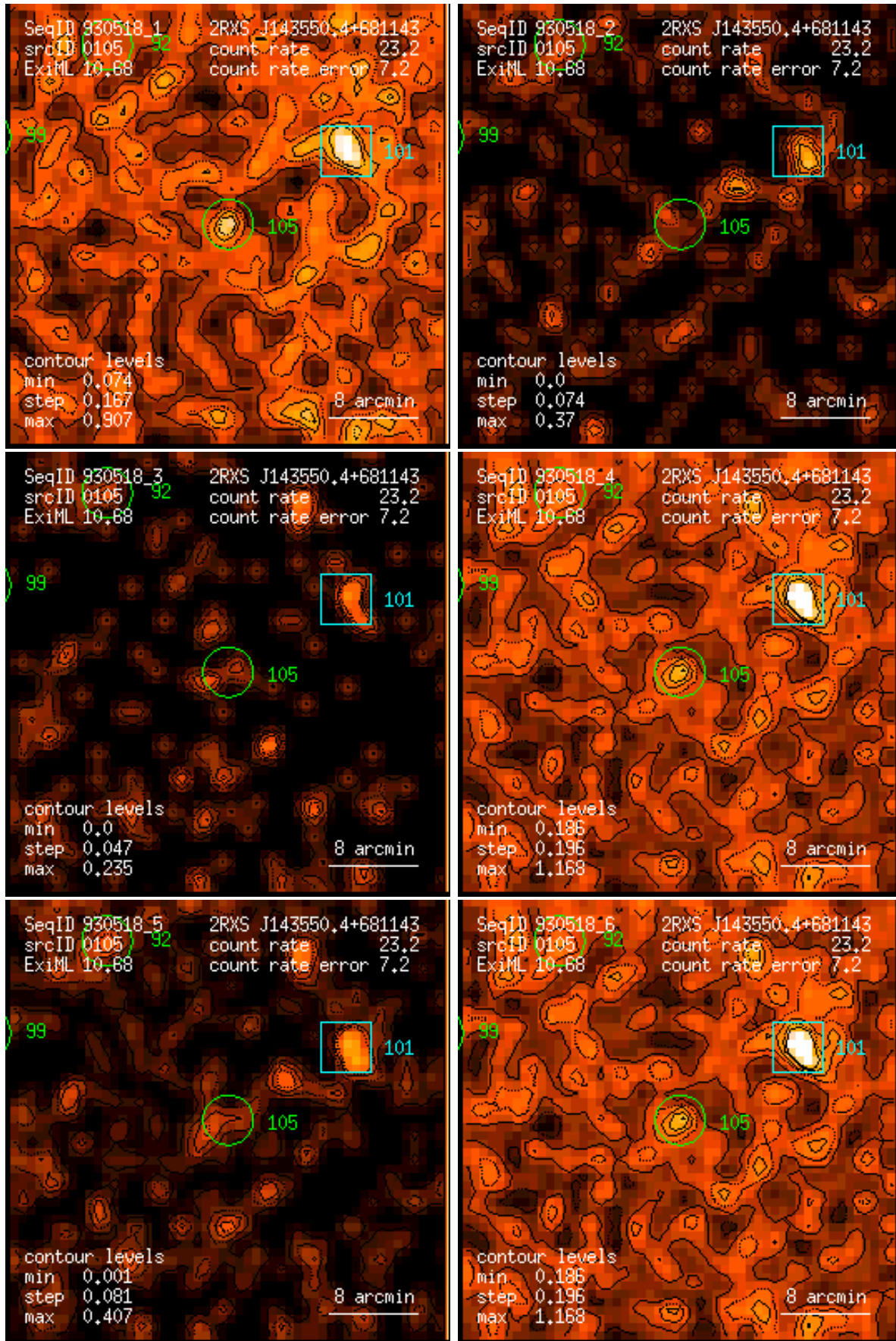
Figure 105: RASS 930518: detection 0105: band rate images, Gaussian filter: (1) PSPC channels 11 – 41, (2) 52 – 90, (3) 91 – 201, (4) 11 – 235, (5) 52 – 201, (6) 11 – 201. Broad band rates in counts/ks. Band rate contour levels in counts/ks/arcmin 2 .
