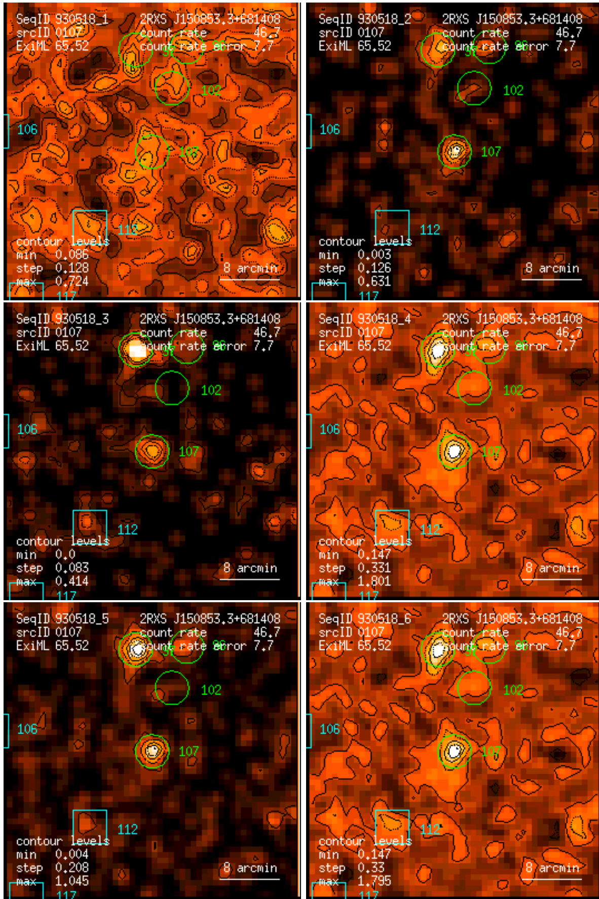
Figure 107: RASS 930518: detection 0107: band rate images, Gaussian filter: (1) PSPC channels 11 – 41, (2) 52 – 90, (3) 91 – 201, (4) 11 – 235, (5) 52 – 201, (6) 11 – 201. Broad band rates in counts/ks. Band rate contour levels in counts/ks/arcmin 2 .
