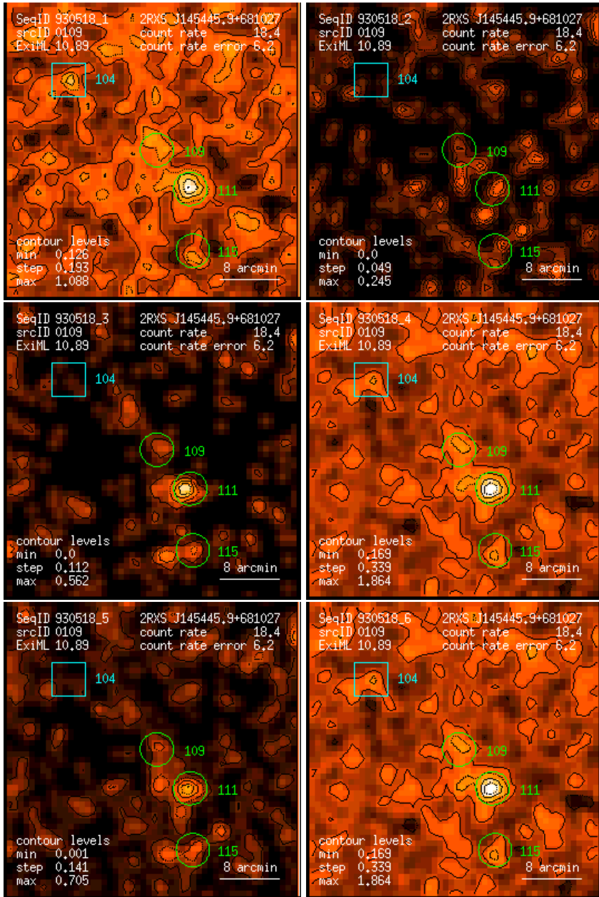
Figure 109: RASS 930518: detection 0109: band rate images, Gaussian filter: (1) PSPC channels 11 – 41, (2) 52 – 90, (3) 91 – 201, (4) 11 – 235, (5) 52 – 201, (6) 11 – 201. Broad band rates in counts/ks. Band rate contour levels in counts/ks/arcmin 2 .
